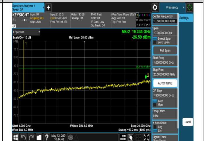
Band66-1.4MHz-16QAM-132665-1RB#0-Range2:1000
