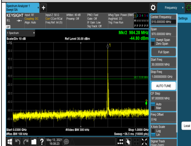
Band17-5MHz-16QAM-23825-1RB#0-Range1:30~1
