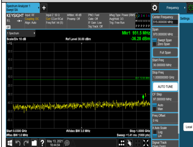
Band66-1.4MHz-16QAM-131979-1RB#0-Range1:30~1000MHz
