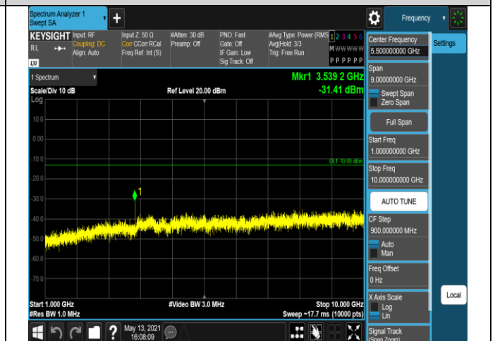
Band17-5MHz-QPSK-23825-1RB#0-Range2:1000~100
