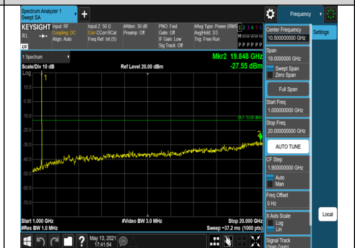
Band66-20MHz-16QAM-132572-1RB#0-Range2:1000~ 20000MHz
