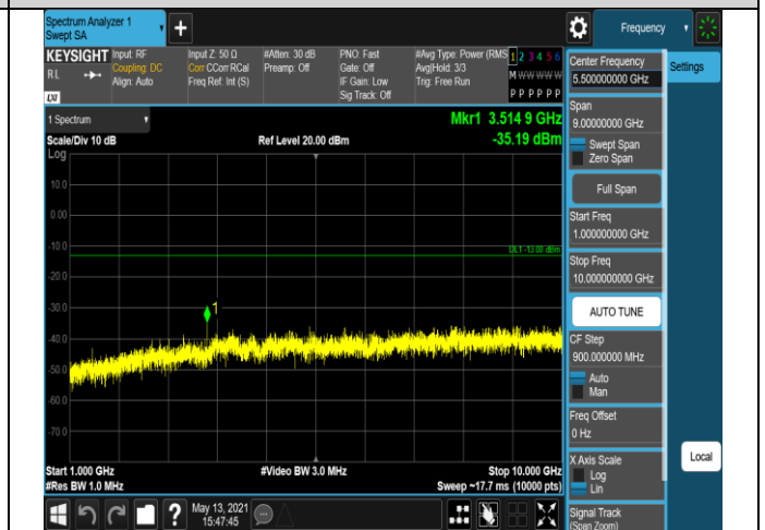
Band12-10MHz-QPSK-23130-1RB#0-Range2:1000~10
