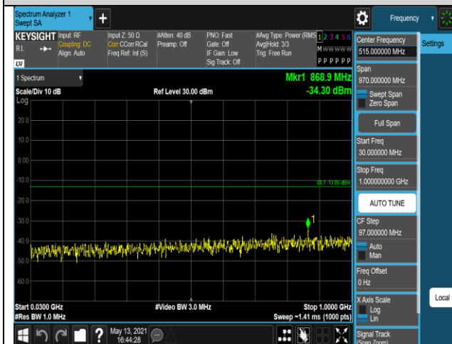
Band66-1.4MHz-16QAM-132665-1RB#0-Range1:30
