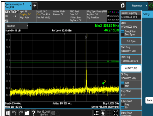
Band17-5MHz-QPSK-23790-1RB#0-Range1:30~10
