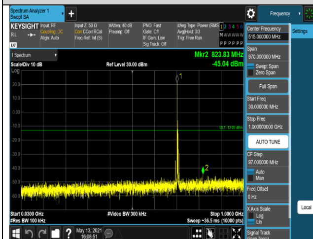
Band17-5MHz-16QAM-23755-1RB#0-Range1:30~1
