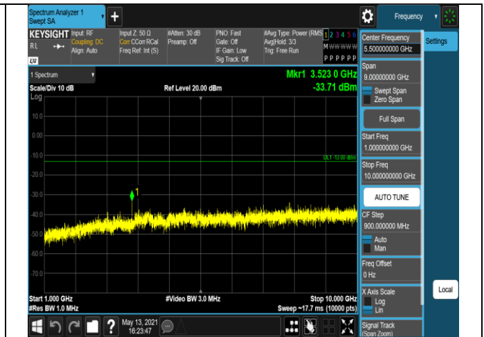
Band17-10MHz-16QAM-23790-1RB#0-Range2:1000~10000MHz
