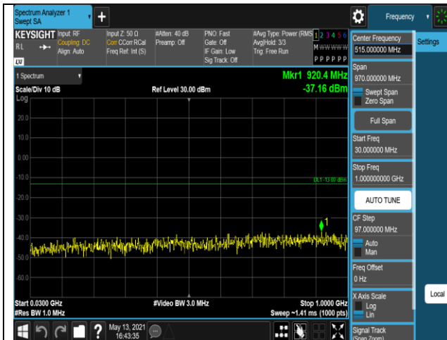
Band66-1.4MHz-16QAM-132322-1RB#0-Range1:30
