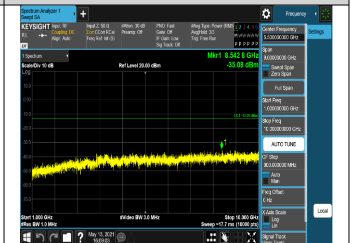
Band17-5MHz-16QAM-23755-1RB#0-Range2:1000~10
