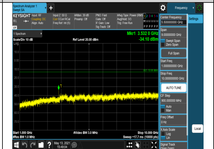
Band17-5MHz-QPSK-23755-1RB#0-Range2:1000~10000MHz
