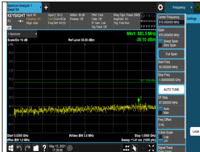
Band66-20MHz-16QAM-132322-1RB#0-Range1:30 ~1000MHz
