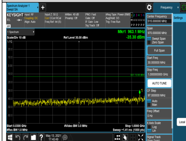
Band66-20MHz-16QAM-132572-1RB#0-Range1:30 ~1000MHz
