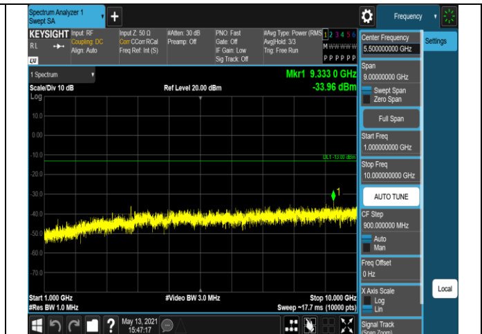
Band12-10MHz-16QAM-23095-1RB#0-Range2:1000~10000MHz
