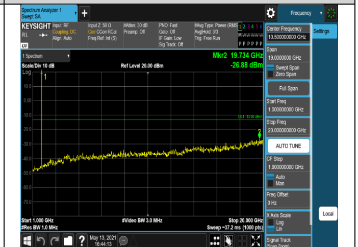
Band66-1.4MHz-QPSK-132665-1RB#0-Range2:1000~20000MHz
