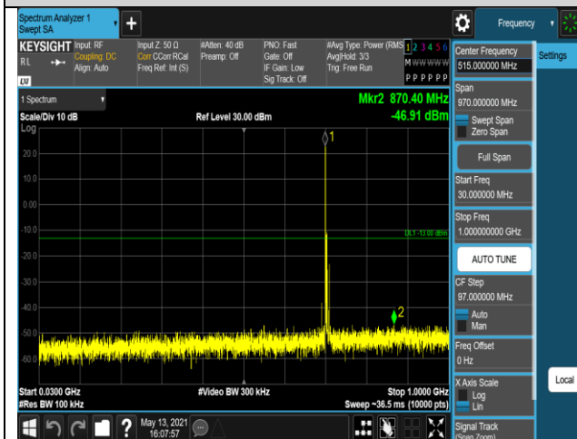
Band17-5MHz-QPSK-23825-1RB#0-Range1:30~10
