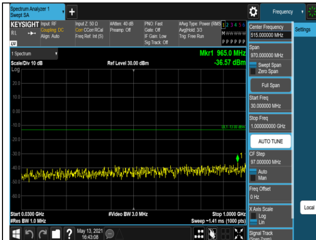
Band66-1.4MHz-QPSK-132322-1RB#0-Range1:30~1000MHz
