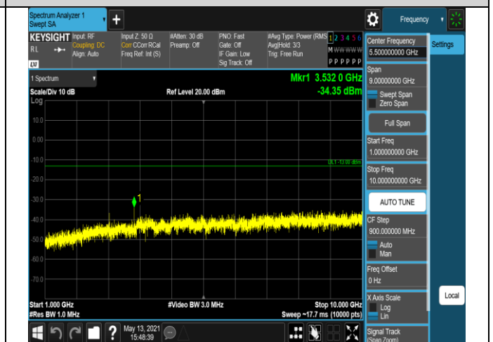
Band12-10MHz-16QAM-23060-1RB#0-Range2:1000~1
