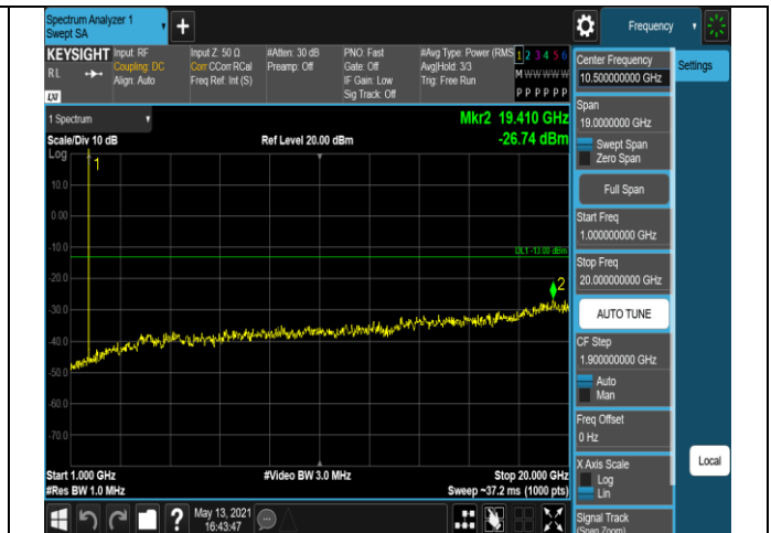
Band66-1.4MHz-16QAM-132322-1RB#0-Range2:1000
