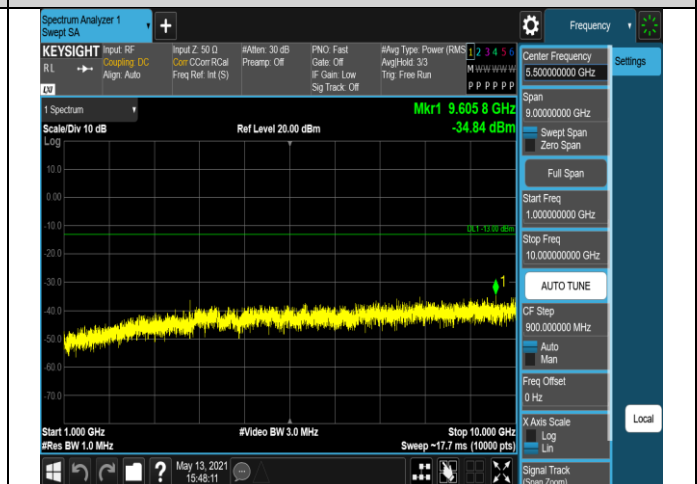
Band12-10MHz-16QAM-23130-1RB#0-Range2:1000~10000MHz
