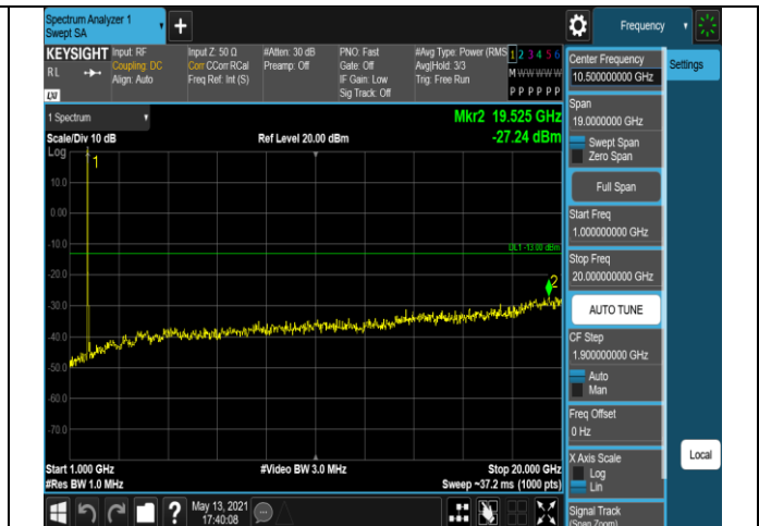
Band66-20MHz-16QAM-132322-1RB#0-Range2:1000~ 20000MHz
