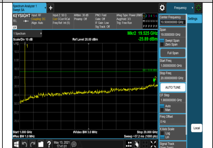
Band66-20MHz-16QAM-132572-1RB#0-Range2:1000~ 20000MHz
