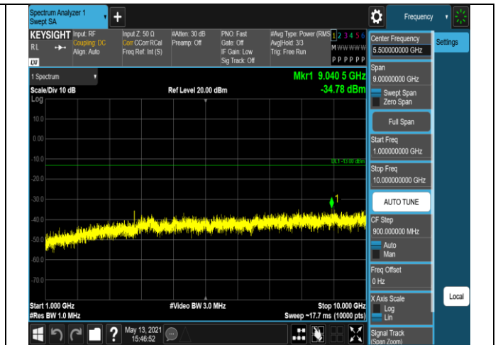
Band12-10MHz-QPSK-23095-1RB#0-Range2:1000~10
