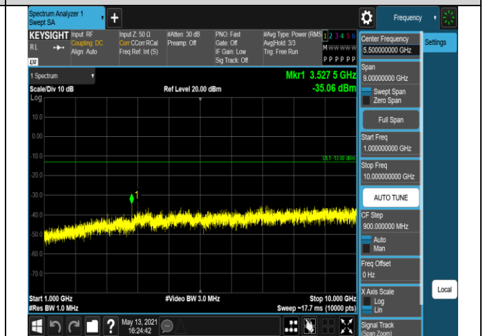
Band17-10MHz-16QAM-23800-1RB#0-Range2:1000~10000MHz
