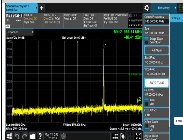
Band17-10MHz-QPSK-23780-1RB#0-Range1:30~1
