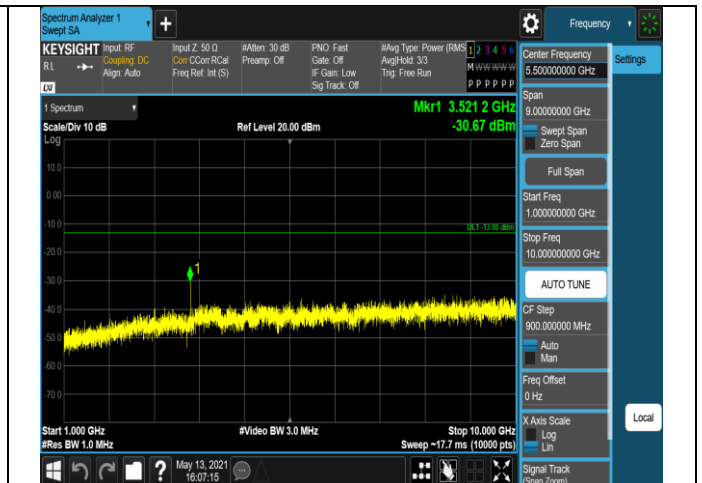
Band17-5MHz-QPSK-23790-1RB#0-Range2:1000~100
