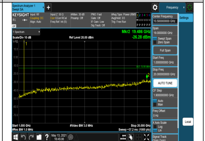
Band66-1.4MHz-16QAM-131979-1RB#0-Range2:1000~20000MHz
