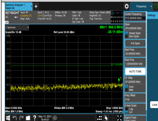
Band66-1.4MHz-QPSK-132665-1RB#0-Range1:30~1000MHz
