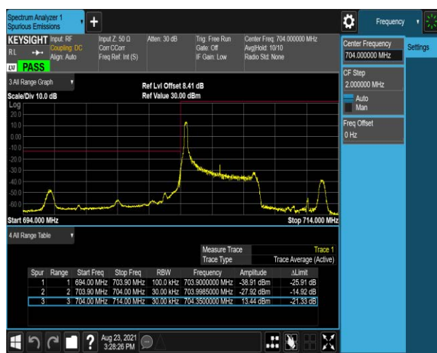
Band17-5MHz-16QAM-23755-25RB#0
