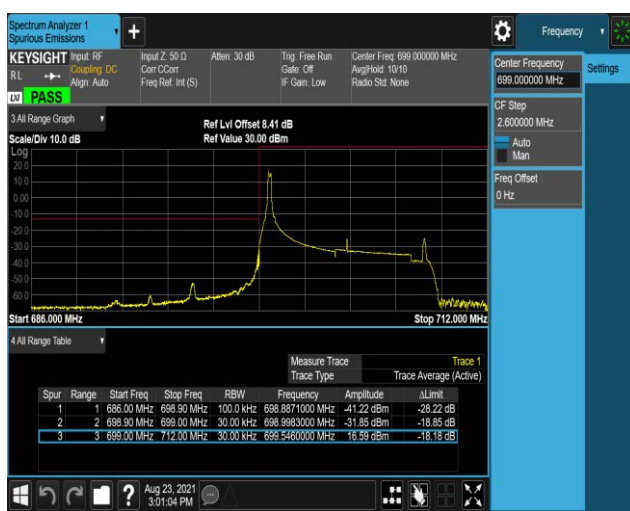
Band12-10MHz-QPSK-23060-50RB#0
