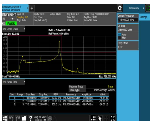
Band12-10MHz-QPSK-23130-1RB#49
