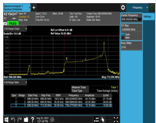
Band12-10MHz-16QAM-23130-1RB#0
