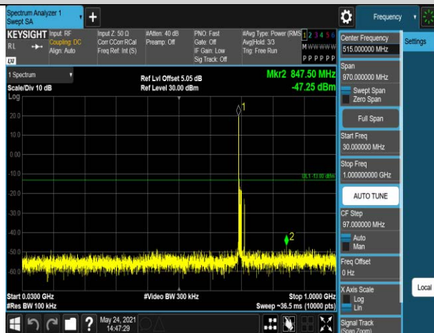
Band12-10MHz-QPSK-23095-1RB#0-Range1:30~1000MHz
