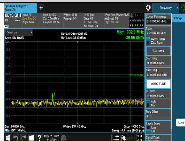
Band2-20MHz-QPSK-18900-1RB#0-Range1:30~10
