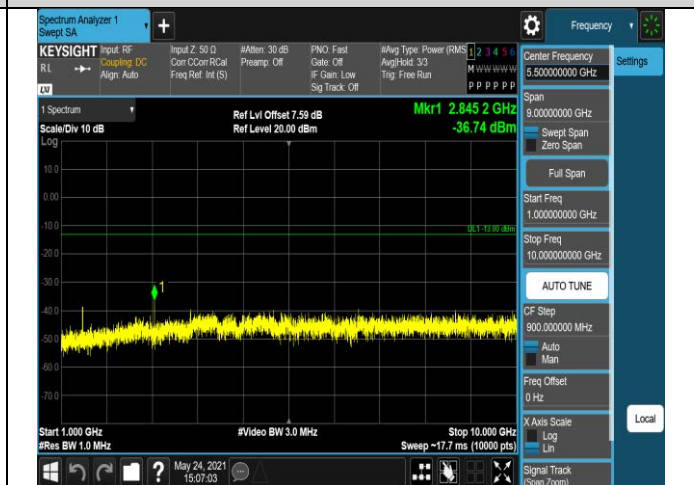
Band17-10MHz-QPSK-23780-1RB#0-Range2:1000~10
