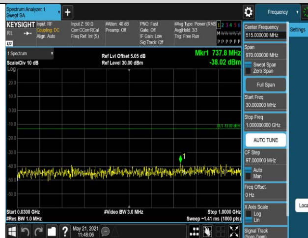
Band2-20MHz-16QAM-18900-1RB#0-Range1:30~1
