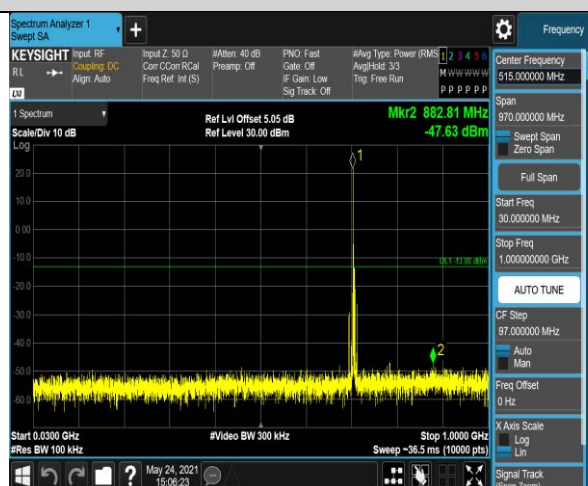
Band17-5MHz-16QAM-23755-1RB#0-Range1:30~1
