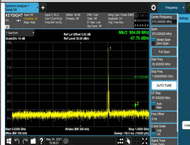
Band17-10MHz-QPSK-23780-1RB#0-Range1:30~1
