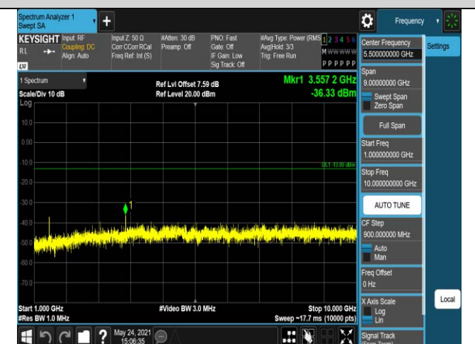
Band17-5MHz-16QAM-23755-1RB#0-Range2:1000~10
