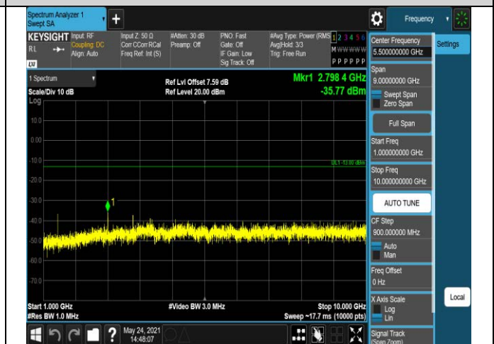
Band12-10MHz-16QAM-23095-1RB#0-Range2:1000~1
