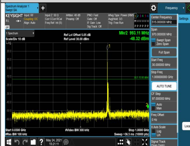
Band17-10MHz-QPSK-23790-1RB#0-Range1:30~1
