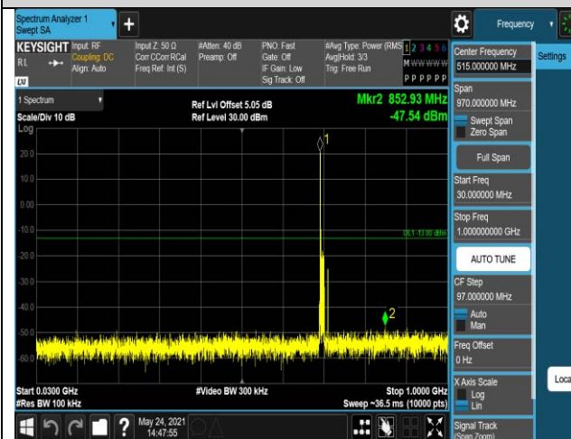
Band12-10MHz-16QAM-23095-1RB#0-Range1:30~1
