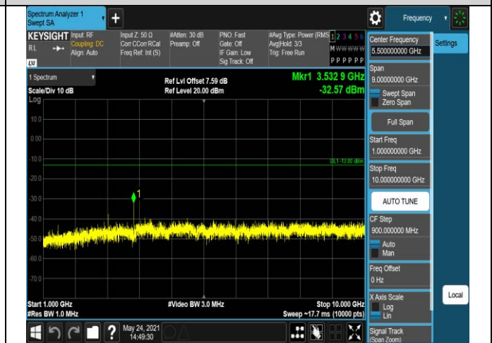
Band12-10MHz-16QAM-23060-1RB#0-Range2:1000~1
