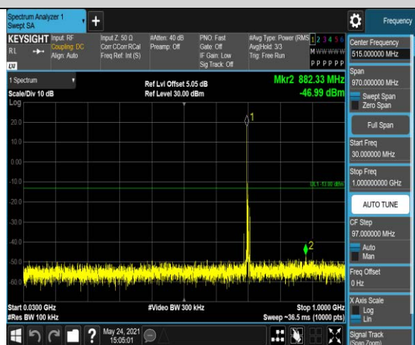
Band17-5MHz-16QAM-23790-1RB#0-Range1:30~1
