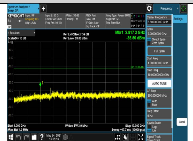
Band17-5MHz-16QAM-23790-1RB#0-Range2:1000~10
