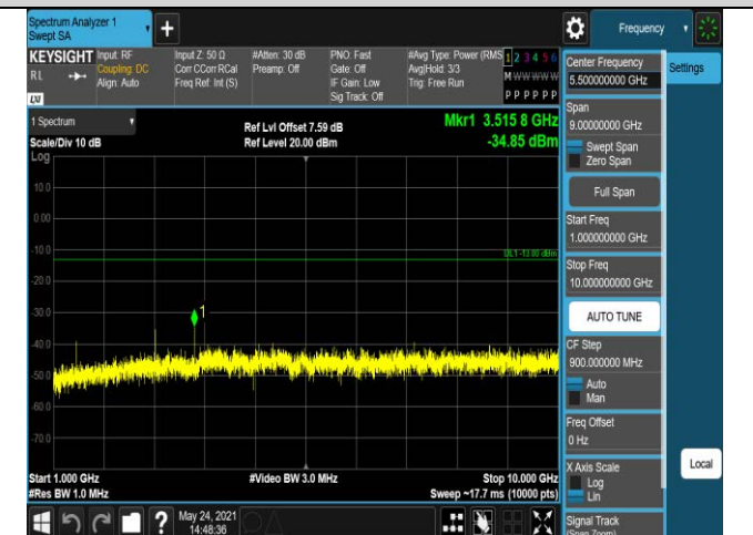
Band12-10MHz-QPSK-23095-1RB#0-Range2:1000~10000MHz
