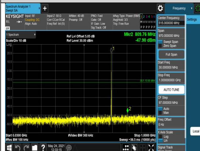
Band12-1.4MHz-16QAM-23095-1RB#0-Range1:30~1
