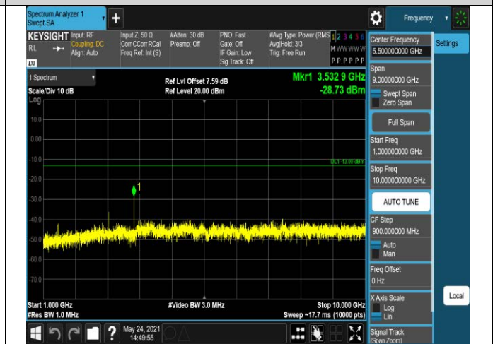
Band17-5MHz-QPSK-23755-1RB#0-Range2:1000~100 00MHz
