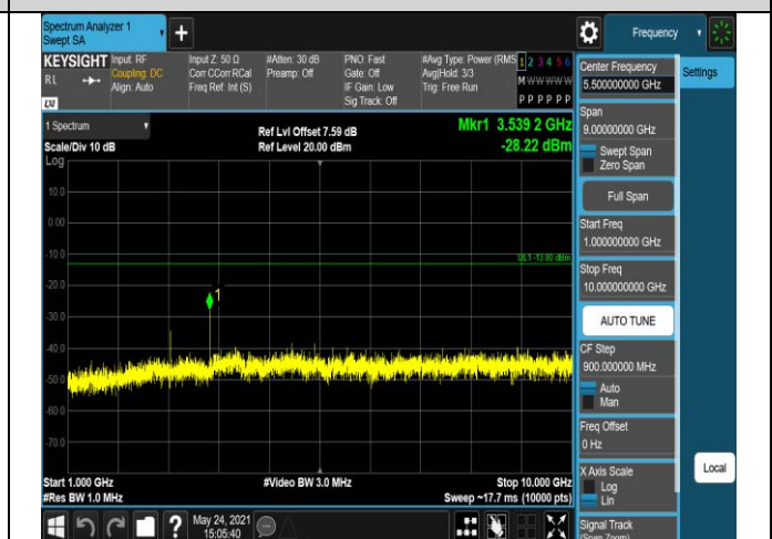
Band17-5MHz-QPSK-23790-1RB#0-Range2:1000~100 00MHz
