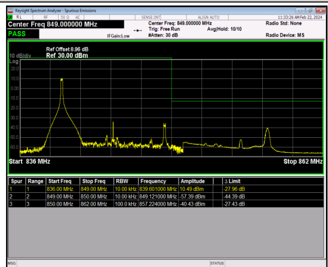
Band5-10MHz-64QAM-20600-50RB#0
