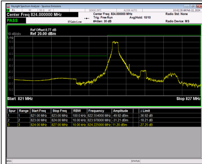
Band5-1.4MHz-64QAM-20407-6RB#0
