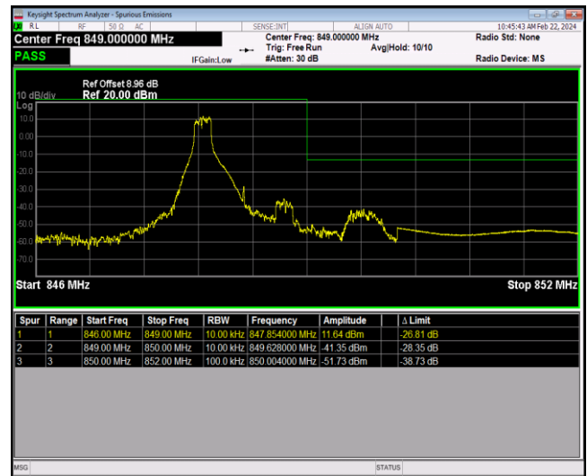
Band5-1.4MHz-64QAM-20643-6RB#0
