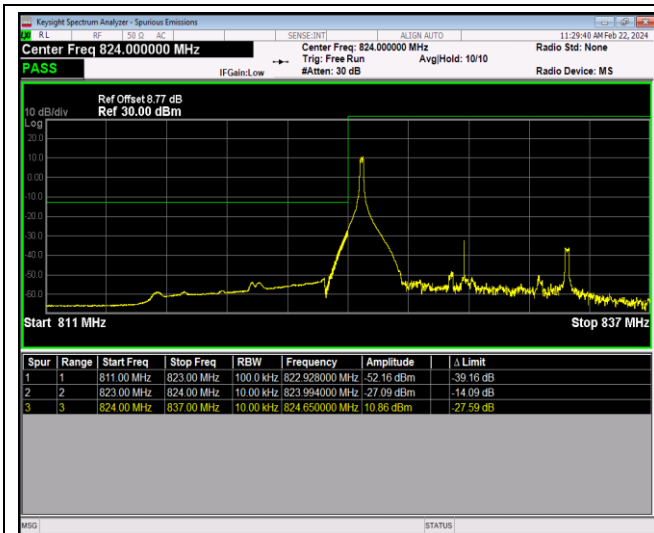
Band5-10MHz-16QAM-20450-50RB#0
