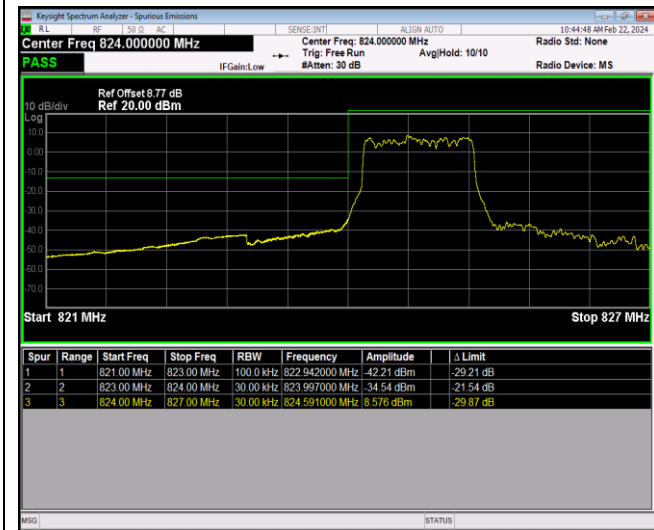
Band5-1.4MHz-64QAM-20643-1RB#5
