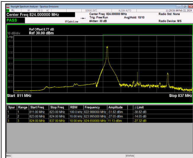
Band5-10MHz-64QAM-20450-50RB#0
