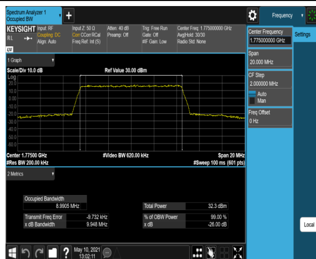
Band66-10MHz-16QAM-132622-50RB#0
