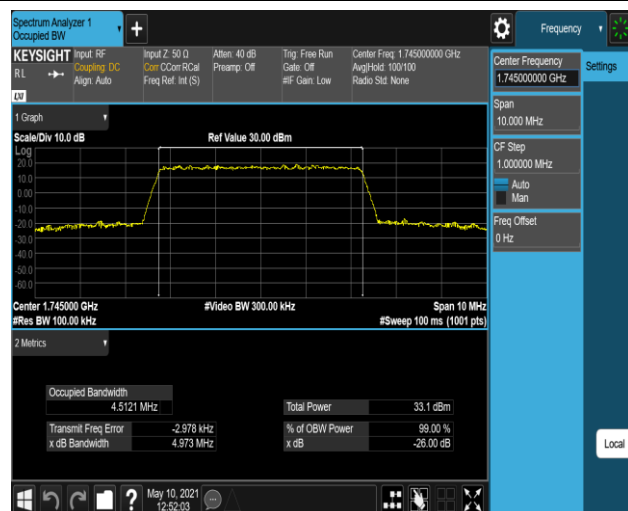
Band66-5MHz-16QAM-131997-25RB#0
