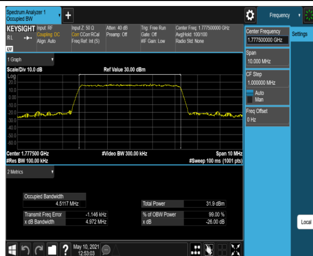
Band66-5MHz-16QAM-132647-25RB#0
