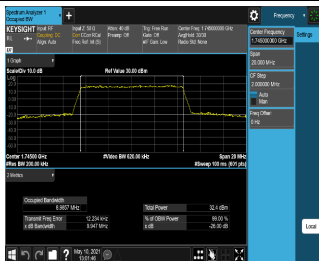
Band66-10MHz-16QAM-132322-50RB#0
