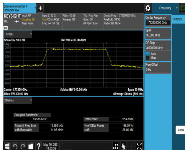
Band66-15MHz-16QAM-132597-75RB#0
