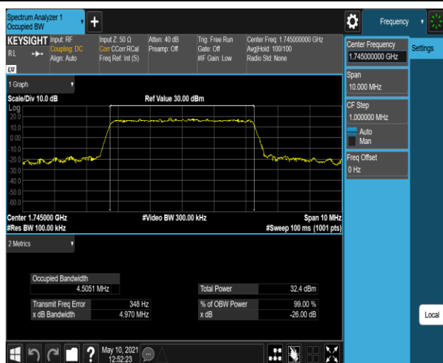
Band66-5MHz-16QAM-132322-25RB#0
