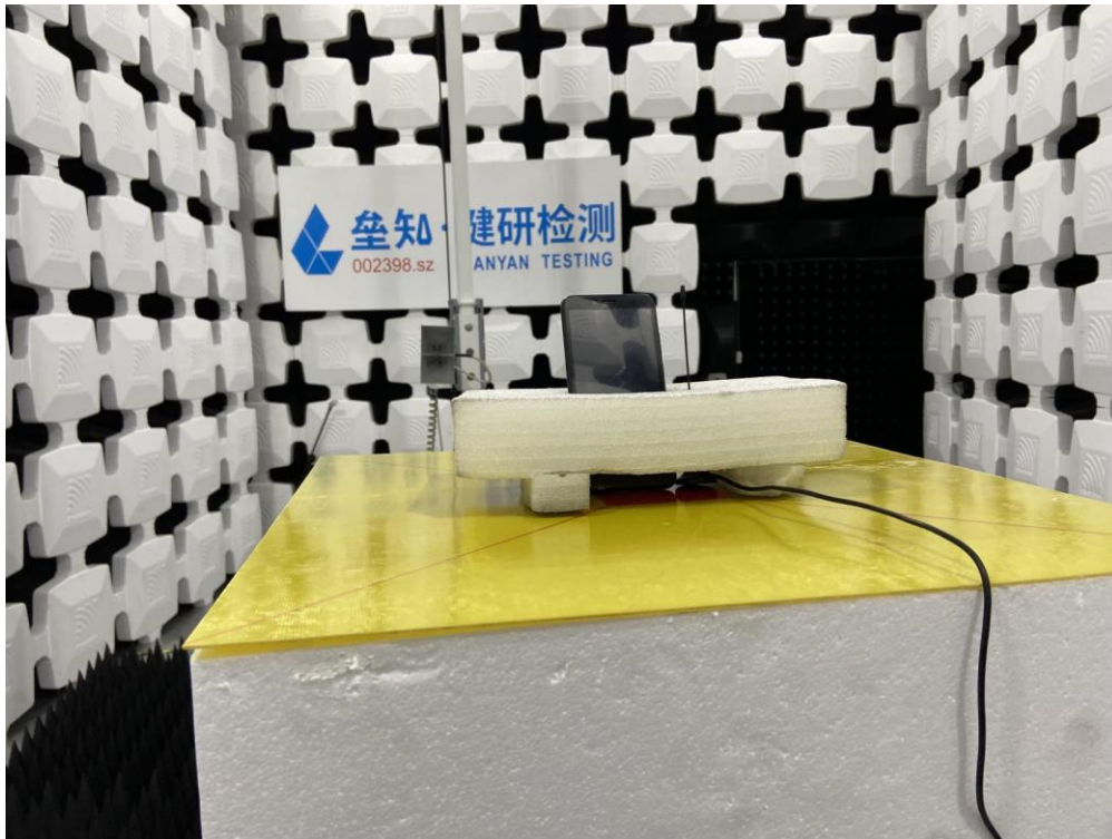
Above 1GHz
