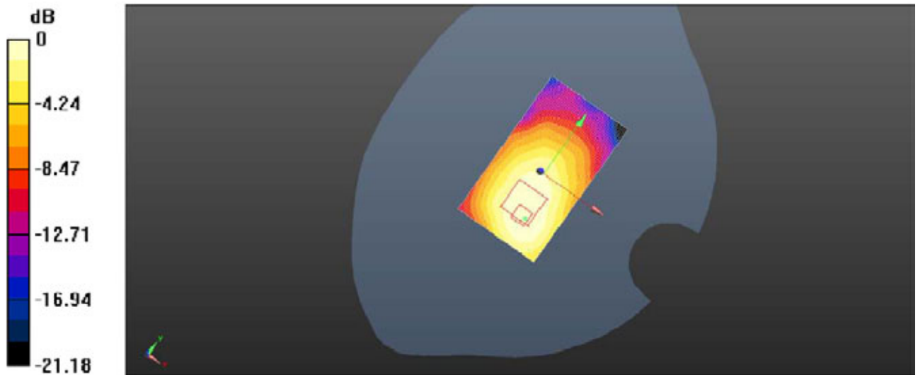
Plot 4: Body Rear Side With Headset (GSM1900 Middle Channel)
