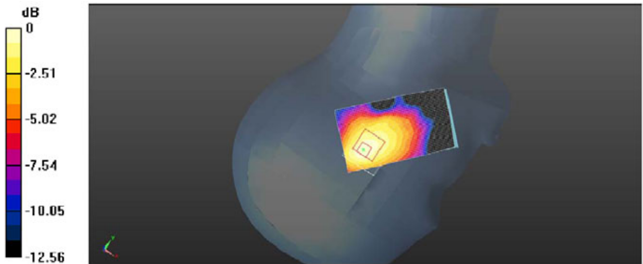
Plot 1: Right Head Touch (GSM850 Middle Channel)
