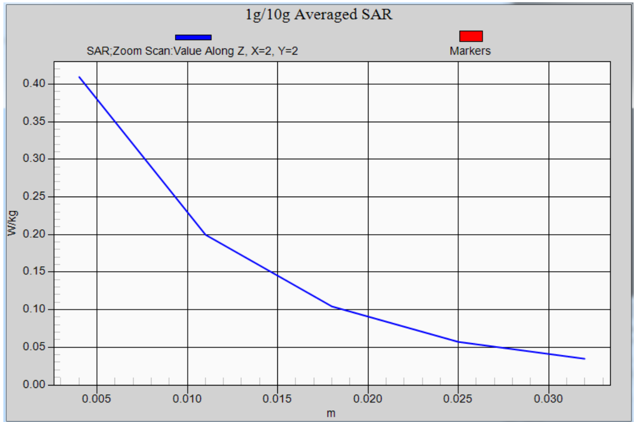
Z-Scan at power reference point- Right Head Touch (GSM1900 Middle Channel)
