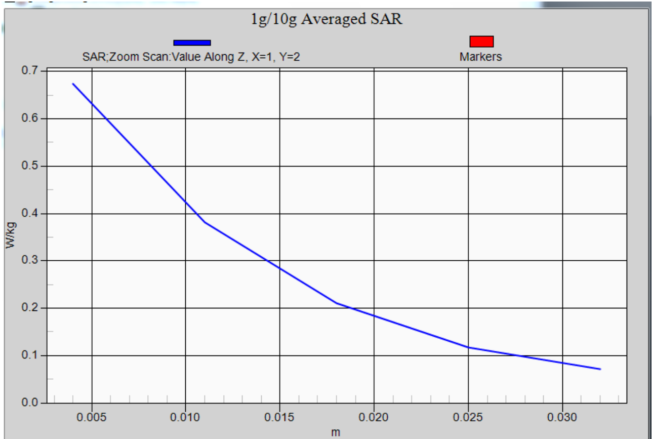
Z-Scan at power reference point- Right Head Touch (GSM850 Middle Channel)
