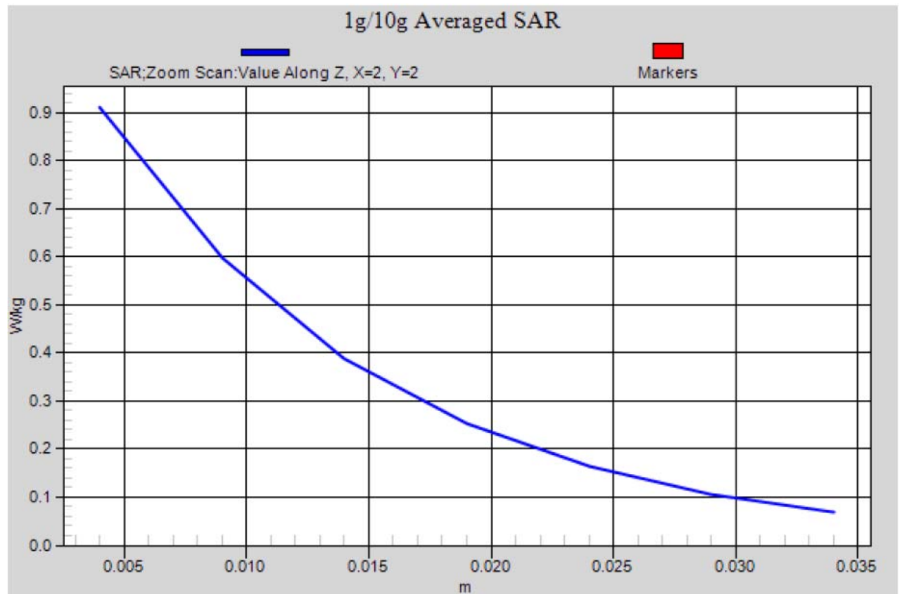
Z-Scan at power reference point- Body Rear Side With Headset (GSM850 Middle Channel)
