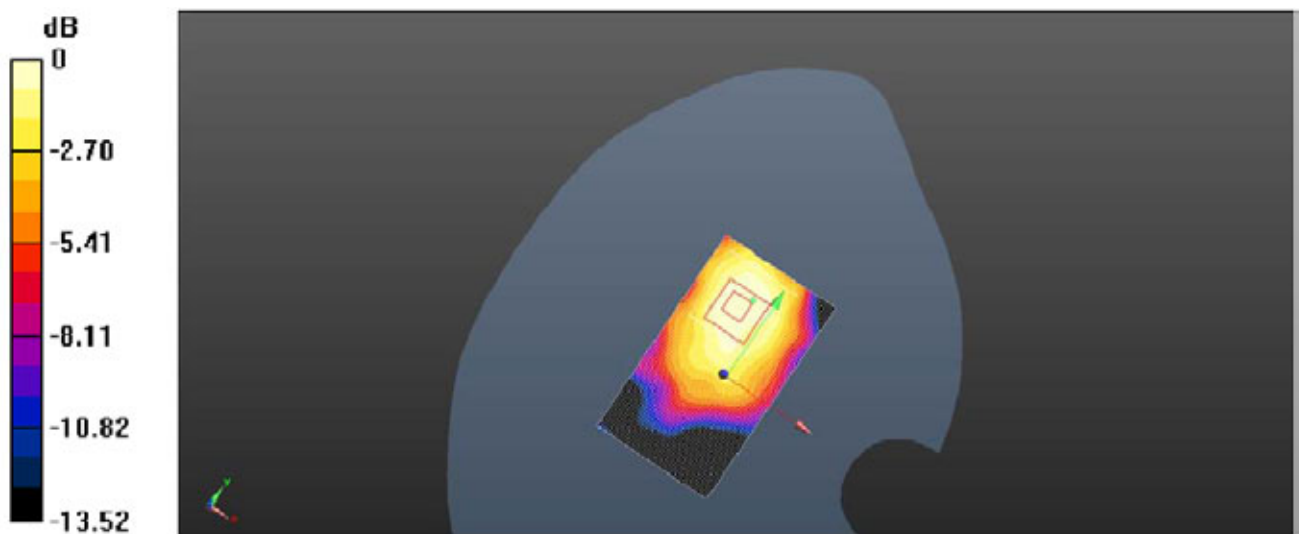
Plot 2: Body Rear Side With Headset (GSM850 Middle Channel)
