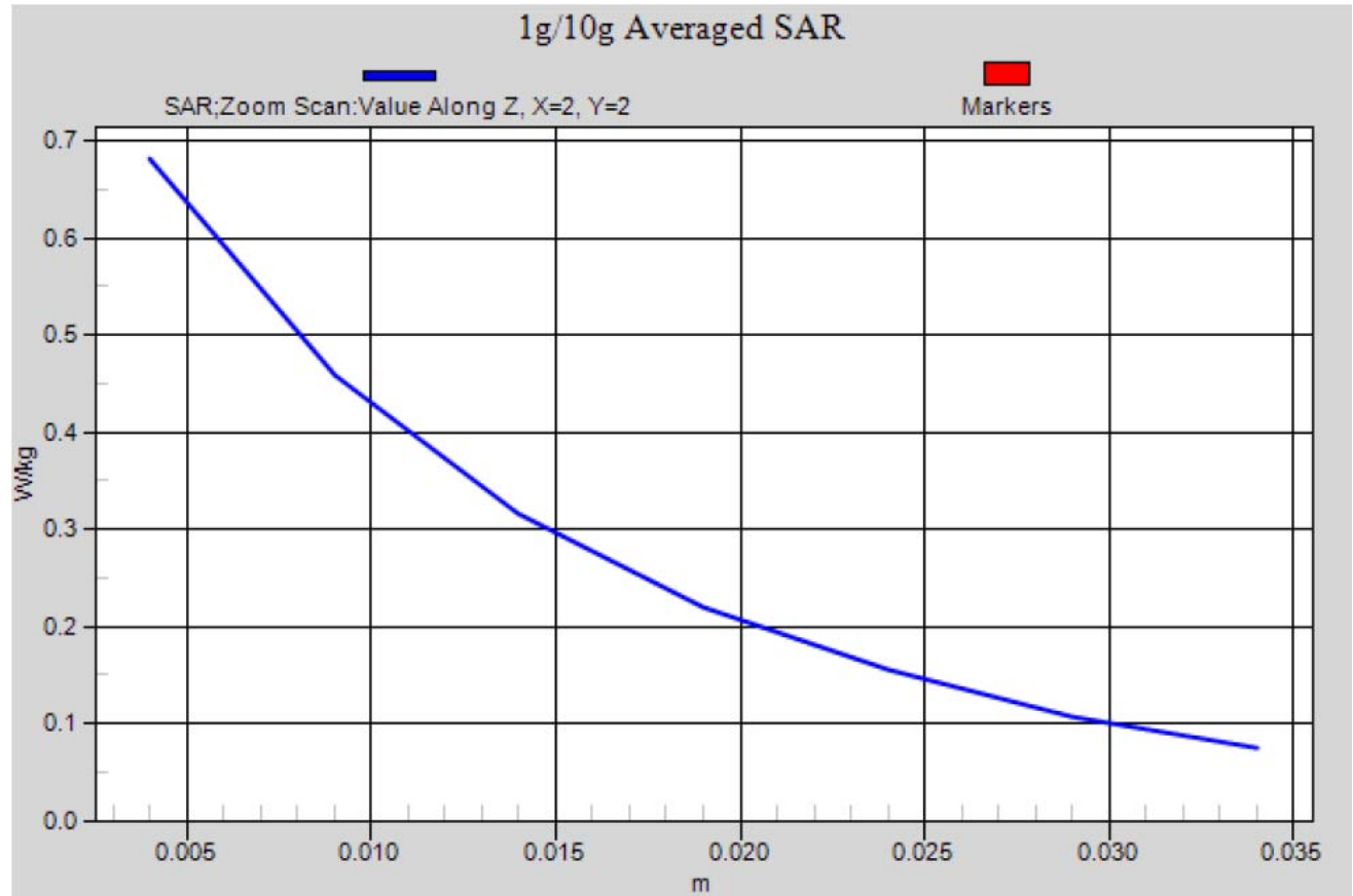
Z-Scan at power reference point- Body Rear Side With Headset (GSM1900 Middle Channel)
