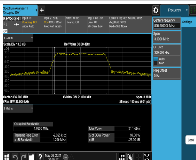
Band5-1.4MHz-16QAM-20525-6RB#0
