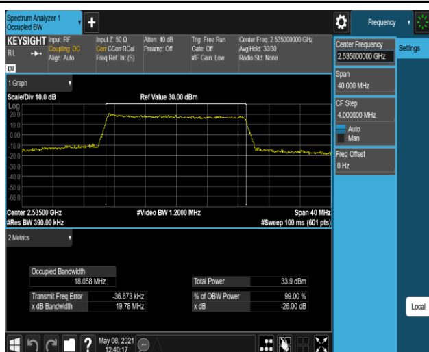
Band7-20MHz-16QAM-21100-100RB#0
