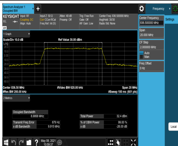
Band5-10MHz-16QAM-20525-50RB#0
