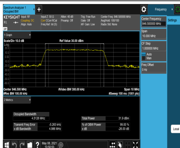
Band5-5MHz-16QAM-20625-25RB#0
