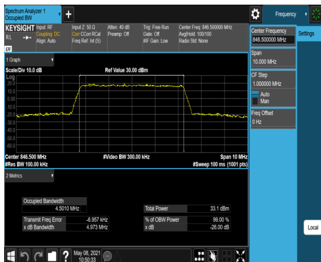
Band5-5MHz-16QAM-20525-25RB#0
