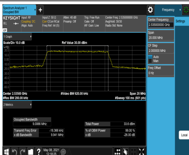
Band7-10MHz-16QAM-21100-50RB#0
