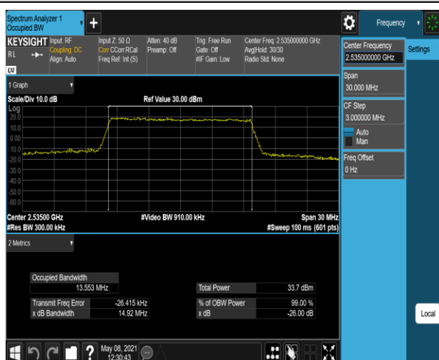
Band7-15MHz-16QAM-21100-75RB#0
