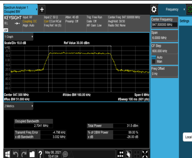
Band5-3MHz-16QAM-20635-15RB#0
