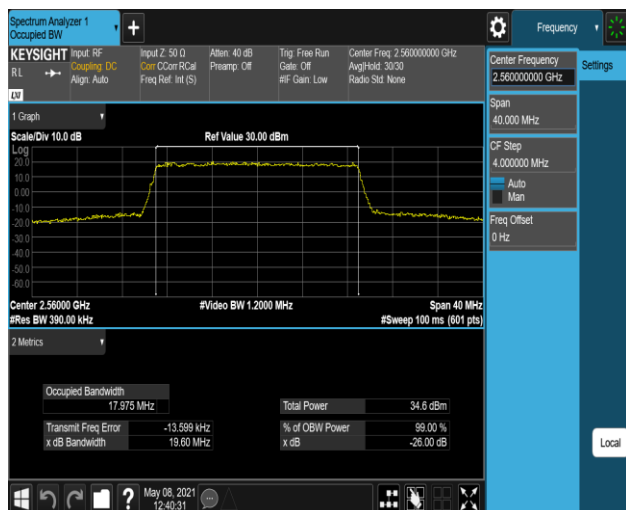
Band7-20MHz-16QAM-21100-100RB#0
