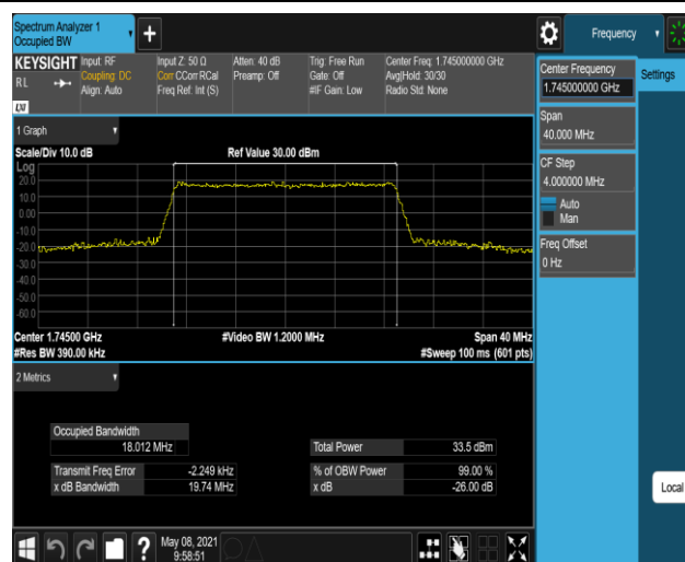
Band4-20MHz-16QAM-20300-100RB#0
