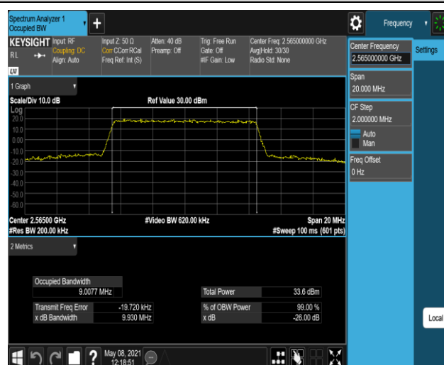
Band7-10MHz-16QAM-21400-50RB#0
