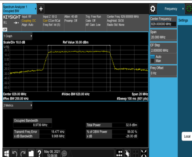
Band5-10MHz-QPSK-20600-50RB#0
