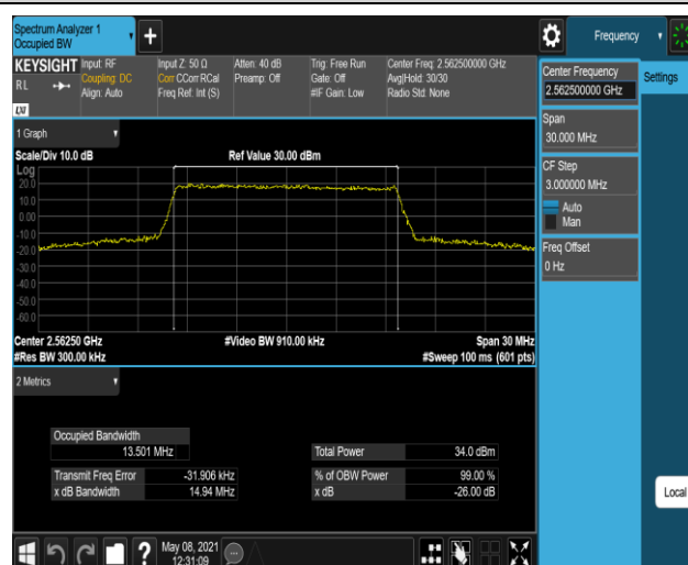
Band7-15MHz-16QAM-21375-75RB#0
