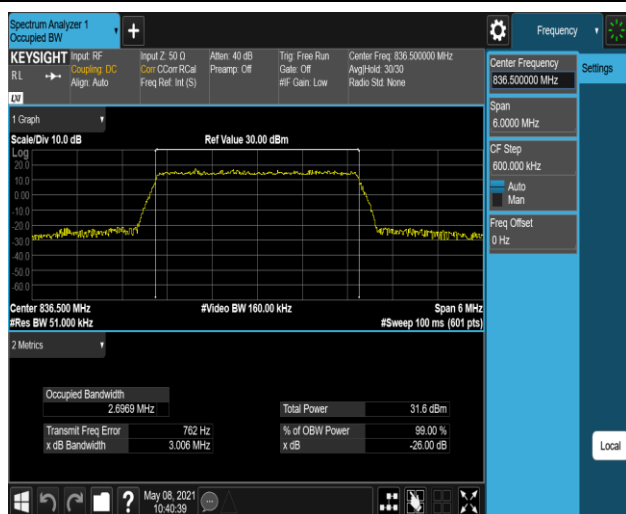
Band5-3MHz-16QAM-20525-15RB#0
