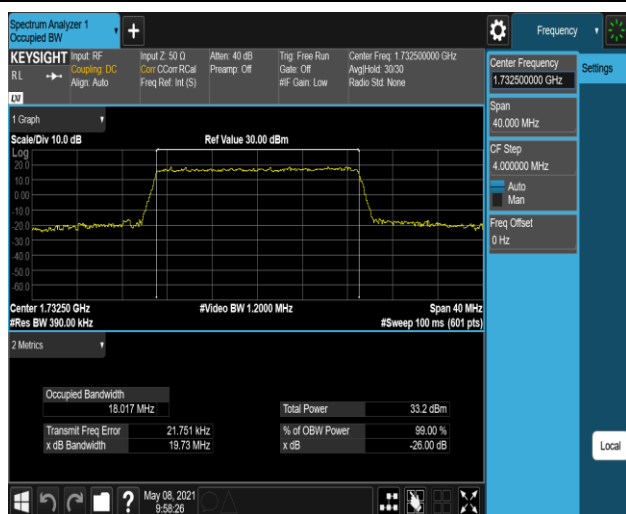
Band4-20MHz-16QAM-20175-100RB#0
