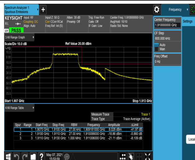
Band2-1.4MHz-16QAM-19193-6RB#0
