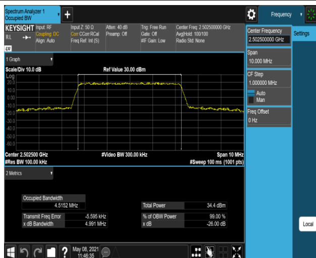
Band7-5MHz-QPSK-21425-25RB#0
