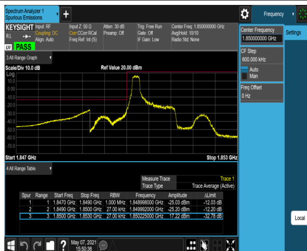
Band2-1.4MHz-16QAM-18607-6RB#0
