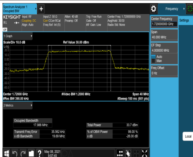
Band4-20MHz-QPSK-20300-100RB#0
