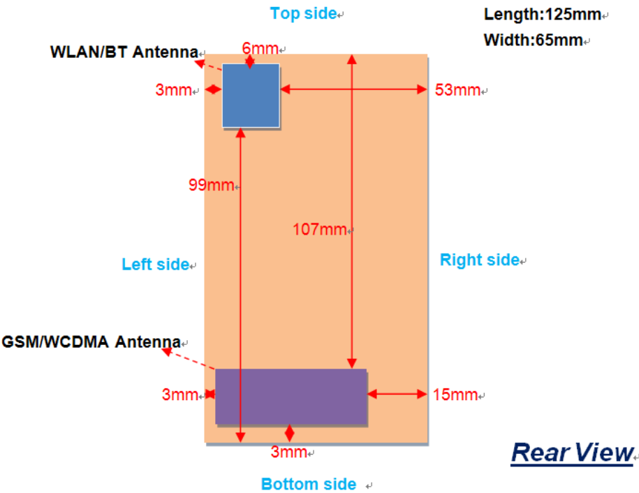
Figure 1:The antenna positions of the DUT
