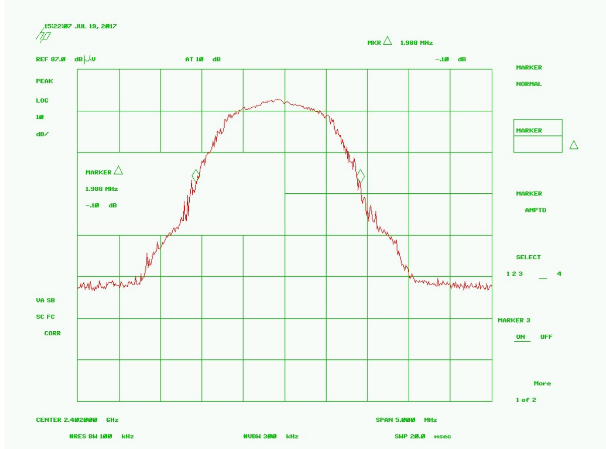
Figure 10. Occupied Bandwidth – Low Channel
