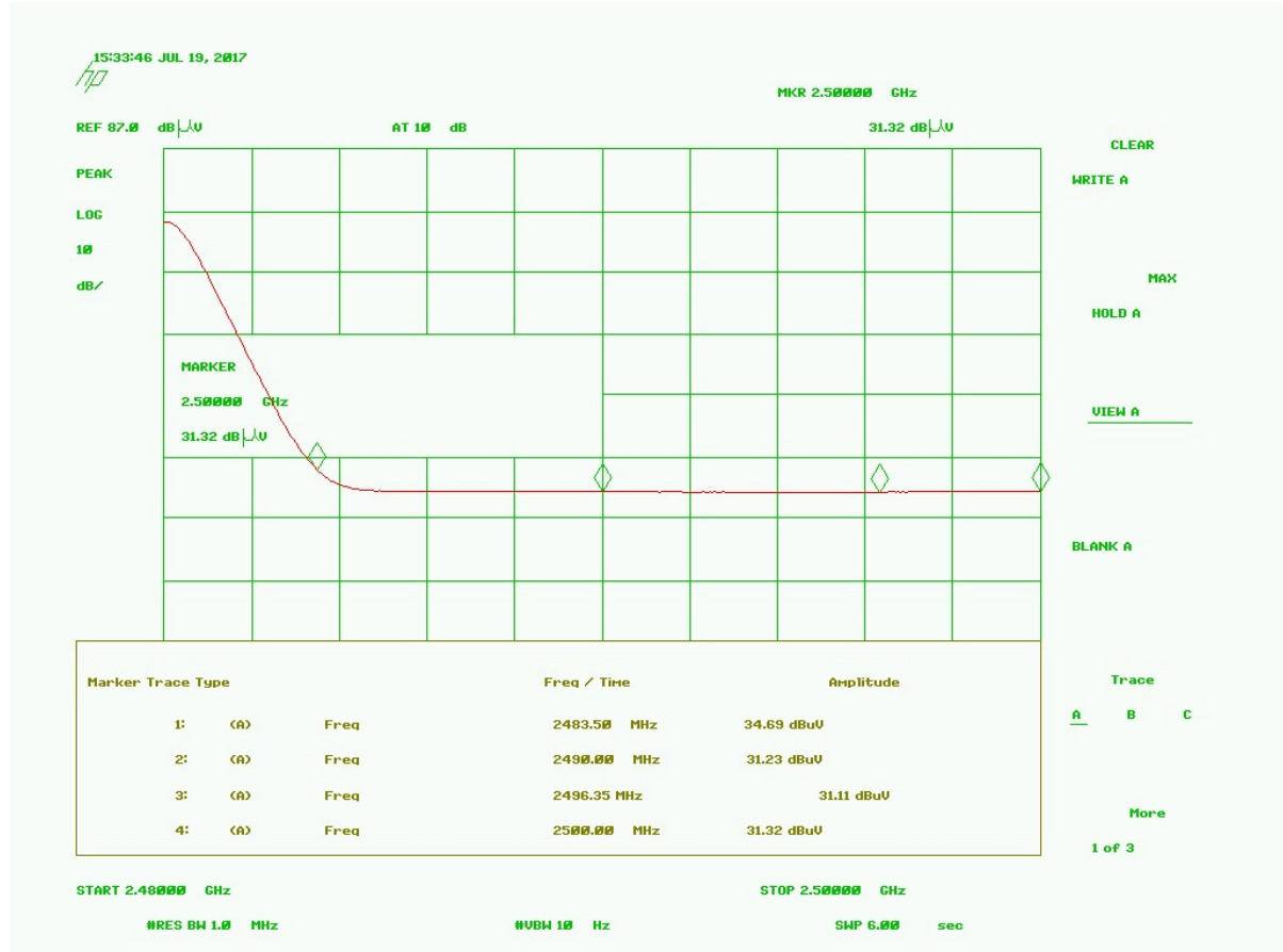
Figure 9. Radiated Restricted Band 2483.5 MHz to 2500 MHz, AVG
