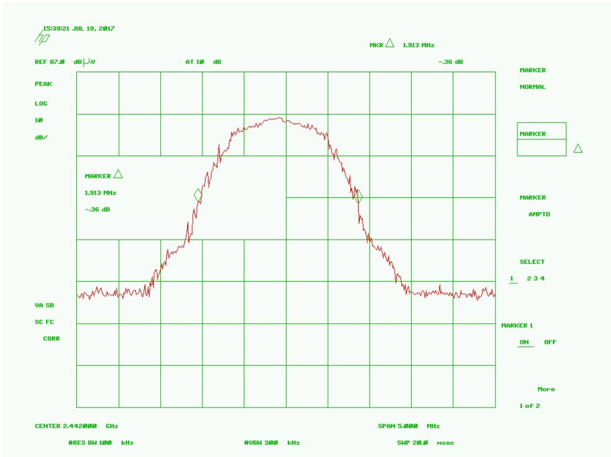
Figure 11. Occupied Bandwidth – Mid Channel
