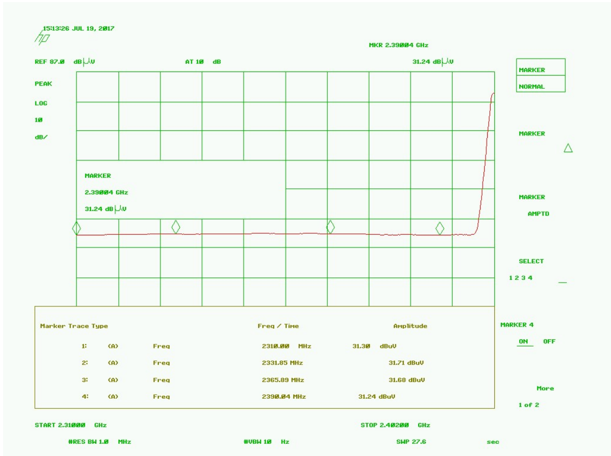
Figure 5. Radiated Restricted Band 2310 MHz to 2390 MHz, AVG
