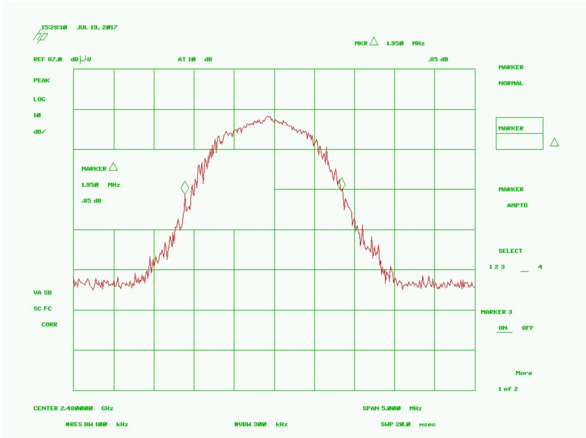
Figure 12. Occupied Bandwidth – High Channel
