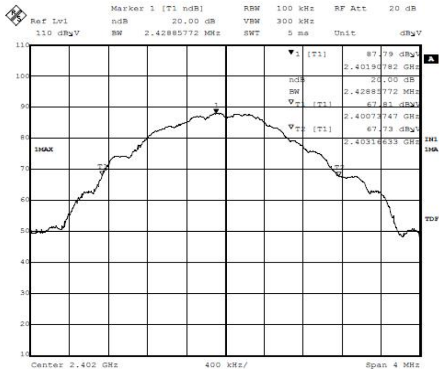
Low Channel – Bandwidth 2.429MHz
