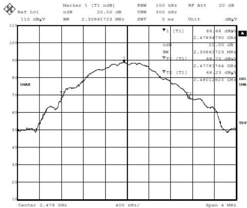
High Channel – Bandwidth 2.309 MHz
