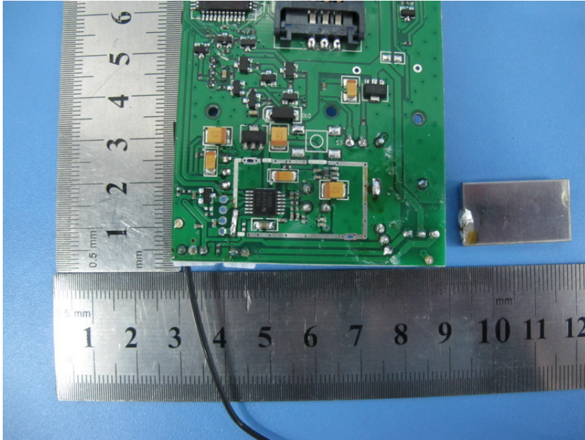
Photo 17 Appearance of PCB
