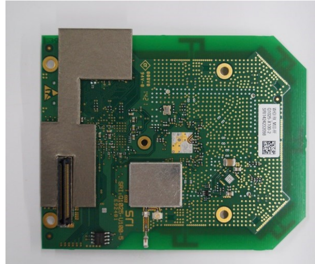
Q1025 – bottom side closed shielding
