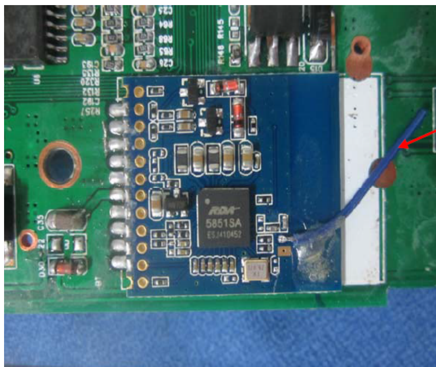
BT Antenna
