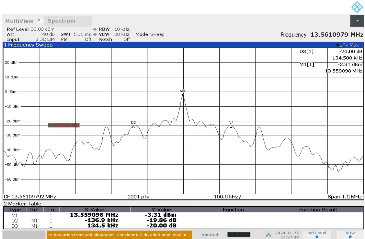
Figure 1 – 20dB Bandwidth
