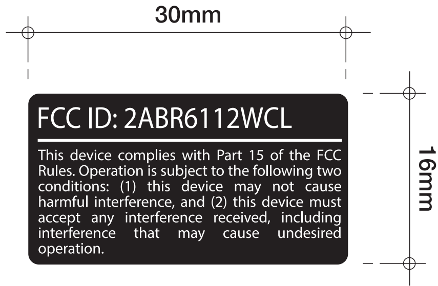
■ FCC LABEL (ENLARGED)
