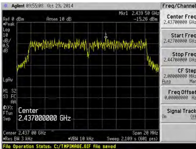
802.11g MID CHANNEL
