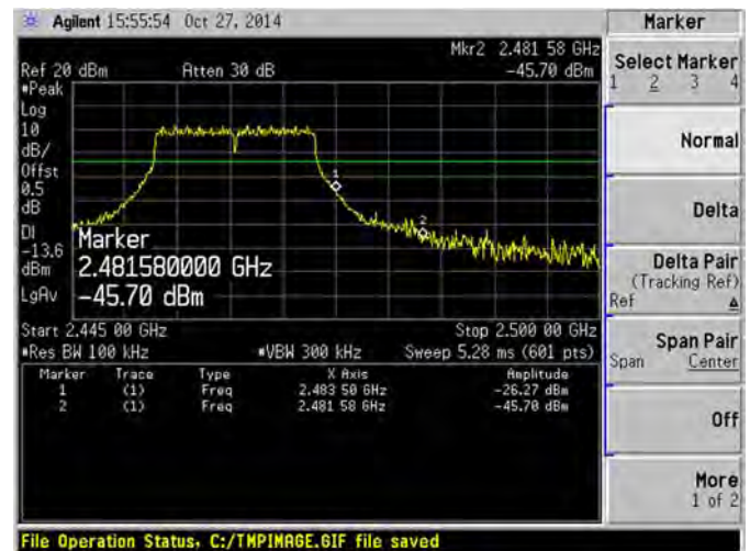
802.11g HIGH CHANNEL, Band Edge
