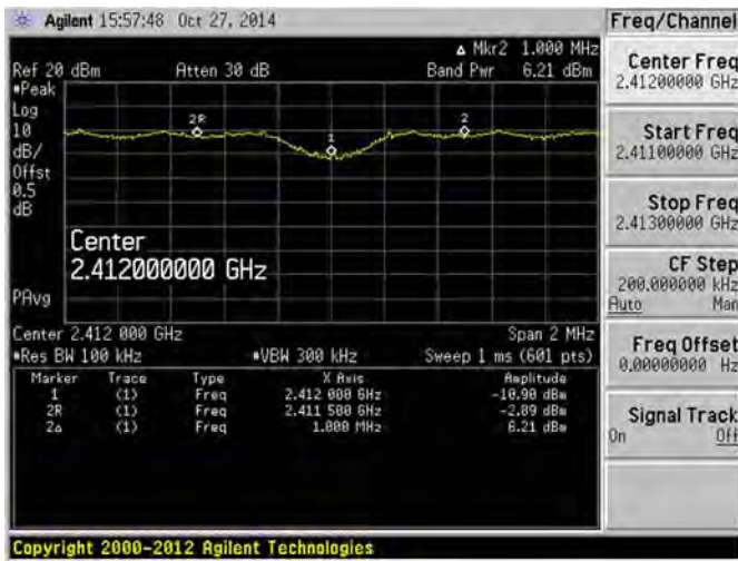
802.11g LOW CHANNEL, Reference level
