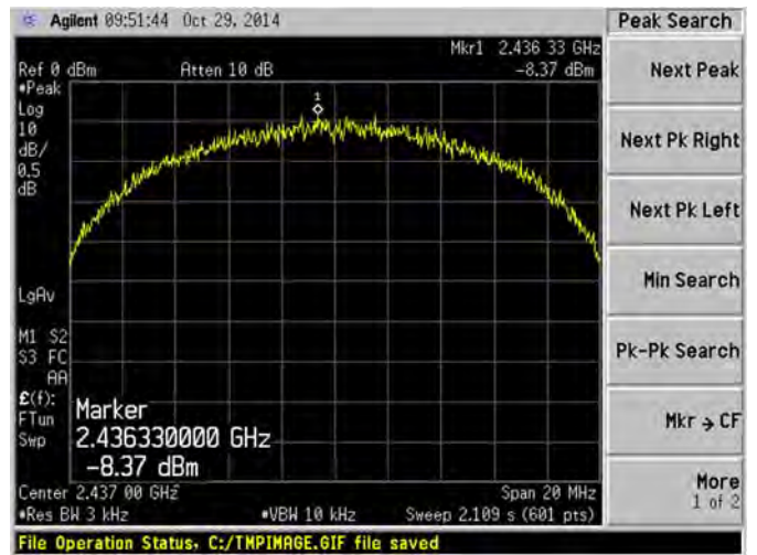
802.11b MID CHANNEL
