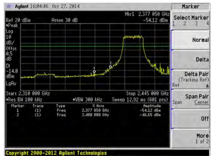
802.11n-20MHz LOW CHANNEL, Band Edge
