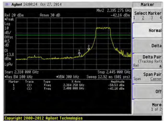
802.11g LOW CHANNEL, Band Edge
