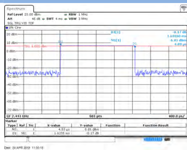
GFSK DH3
