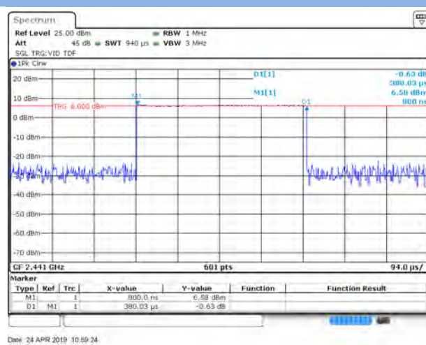
GFSK DH1
