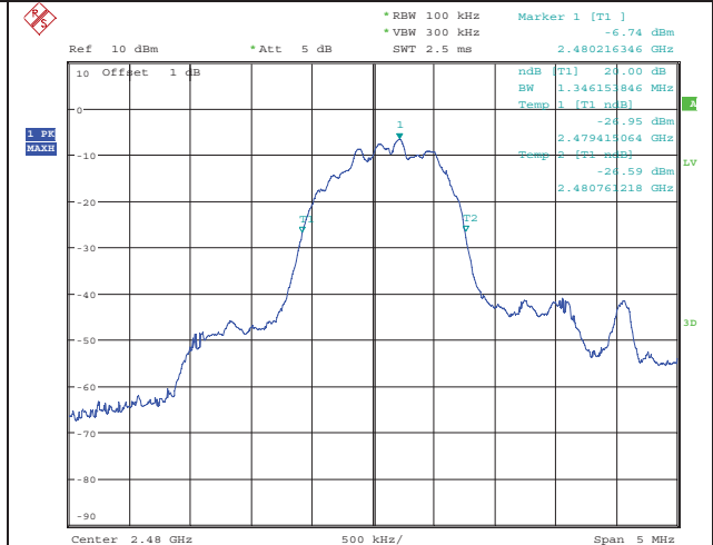
8-DPSK 2480MHz (20dB bandwidth)
