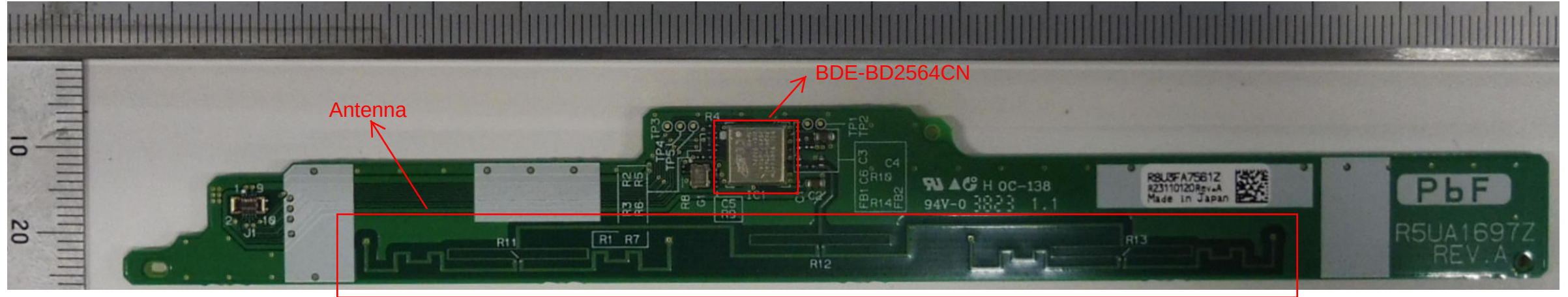
Component Side
