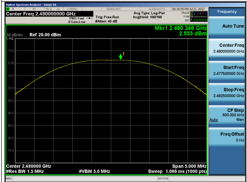
Test_Graph_GFSK_ANT1_2480_125kbps_Peak Power
