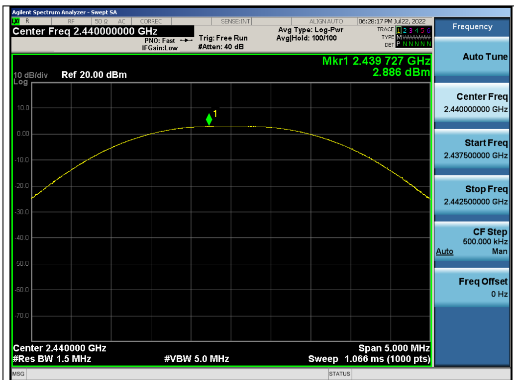
Test_Graph_GFSK_ANT1_2440_125kbps_Peak Power
