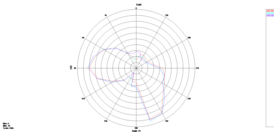
Figure 17: YZ Plane (Phi = 90°)
