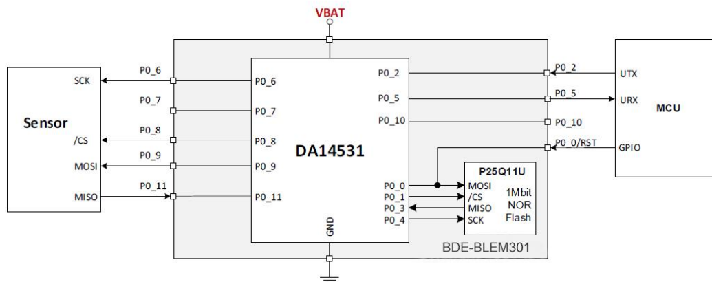
Figure 8: Example of Connecting a Sensor to the SPI Bus and an MCU to RST and UART
