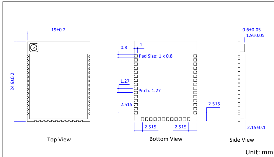
Figure 5-1. Mechanical Drawing
