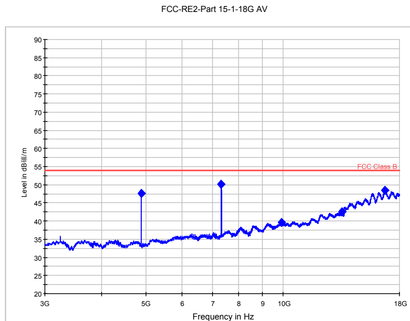
Fig. 27 Radiated Spurious Emission (Ch19, 3 GHz-18 GHz)
