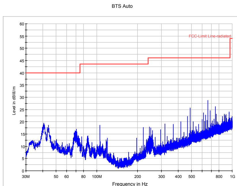
Fig. 28 Radiated Spurious Emission (Ch39, 30 MHz-1 GHz)
