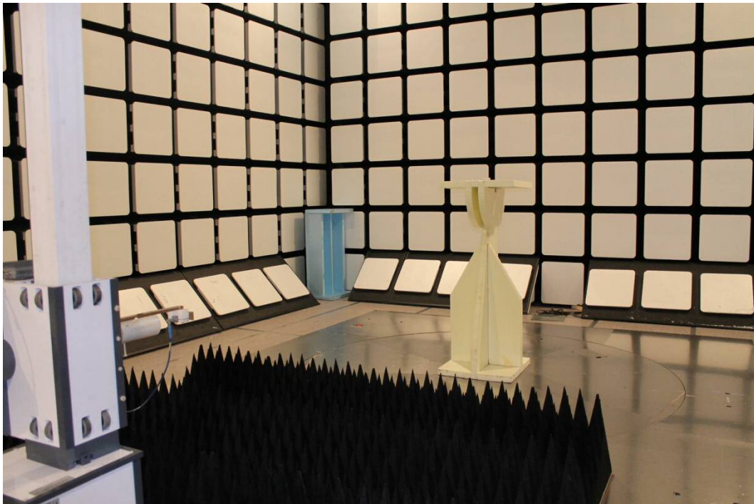
Photograph 4. Radiated emission test set-up (18 - 26 GHz).
