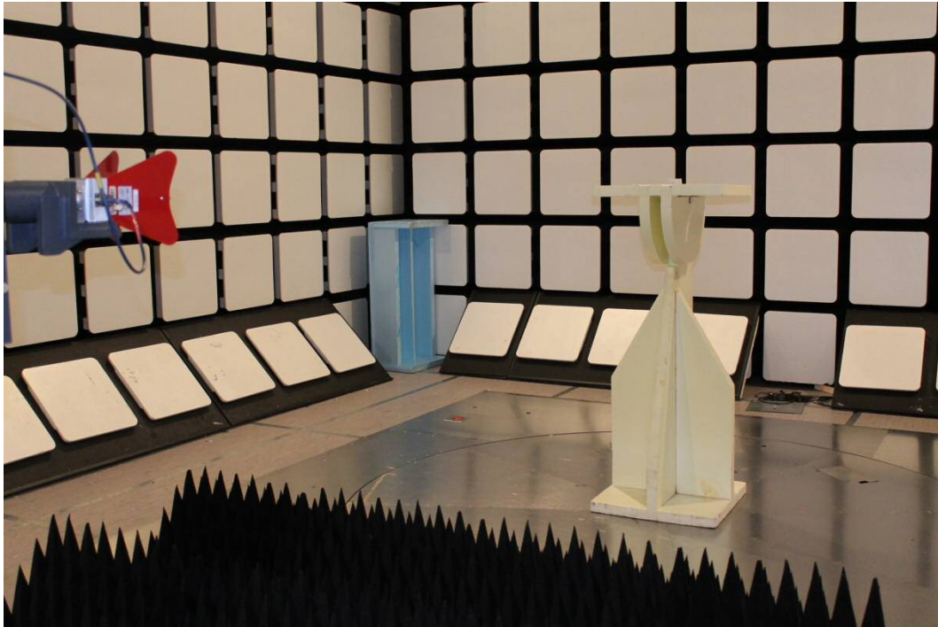
Photograph 3. Radiated emission test set-up (1 – 18 GHz).
