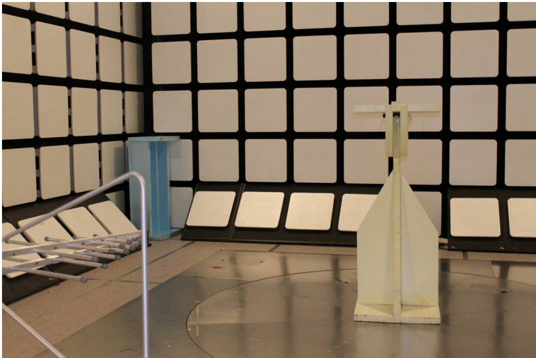
Photograph 2. Radiated emission test set-up (30 – 1000 MHz).
