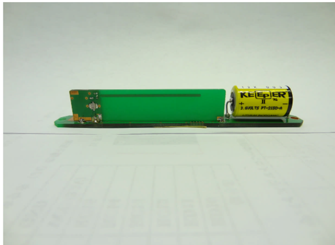
SIDE VIEW 2
