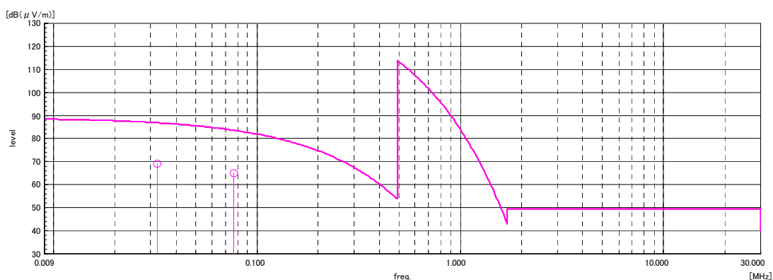
Figure 14 Radiated Emission (Middle ch 9kHz-30MHz)
