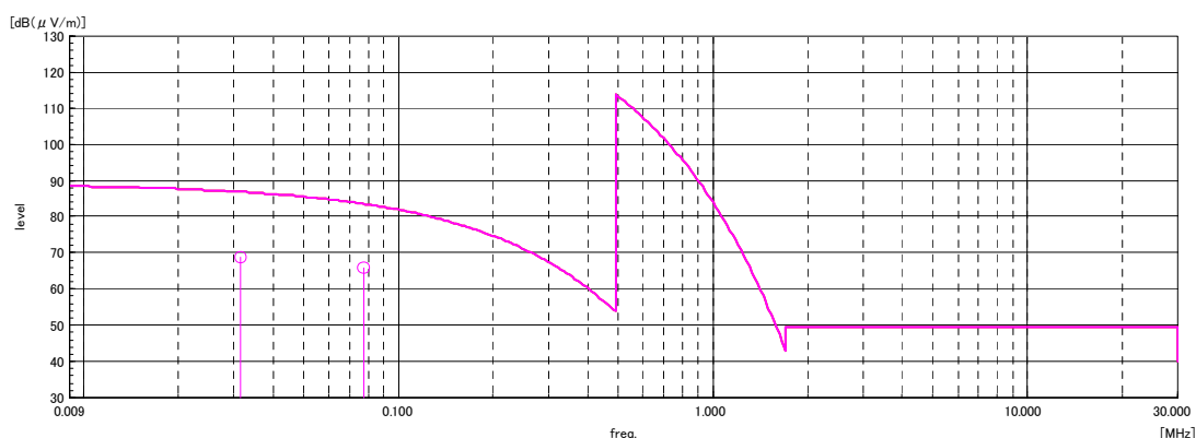
Figure 13 Radiated Emission (Lower ch 9kHz-30MHz)
