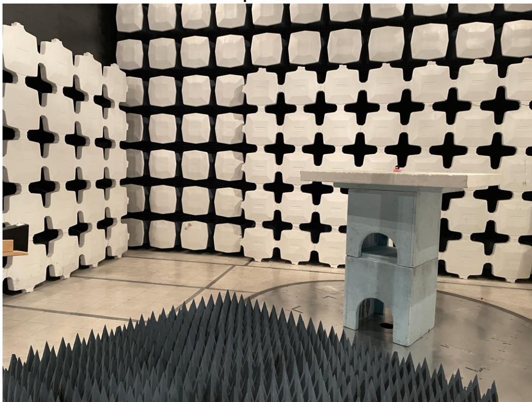
Radiated Emission 18 – 26.5 GHz Test Setup: TX Mode
