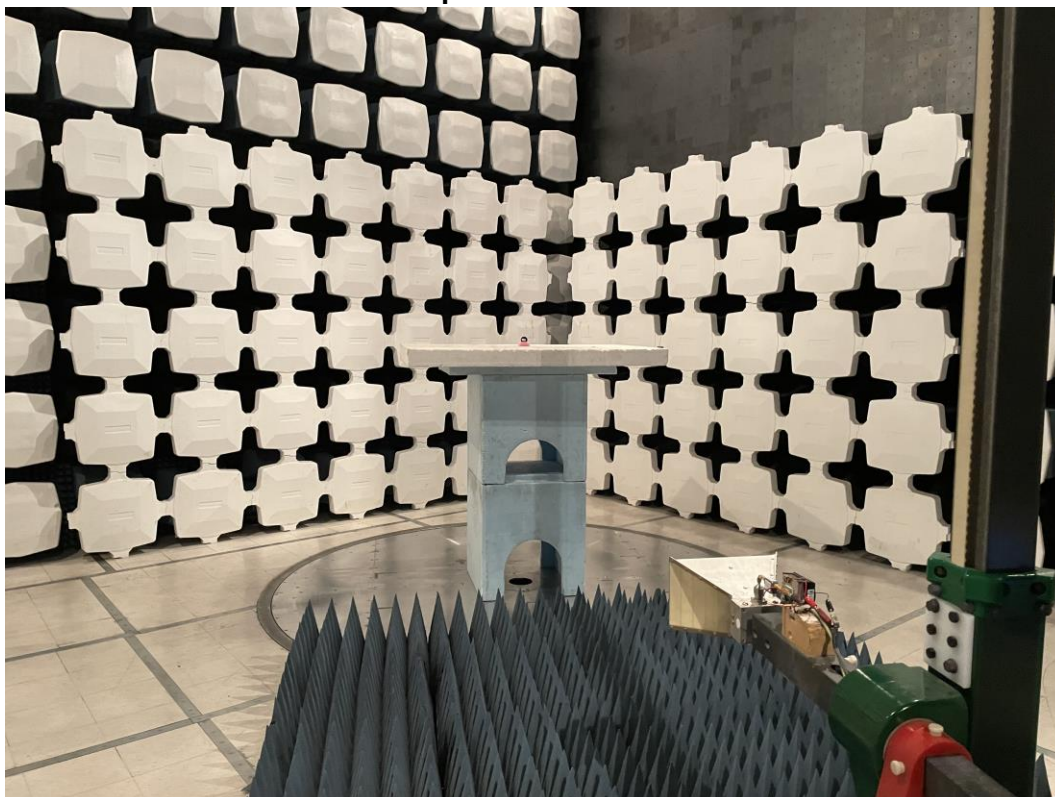
Radiated Emission 1 – 18 GHz Test Setup: TX Mode
