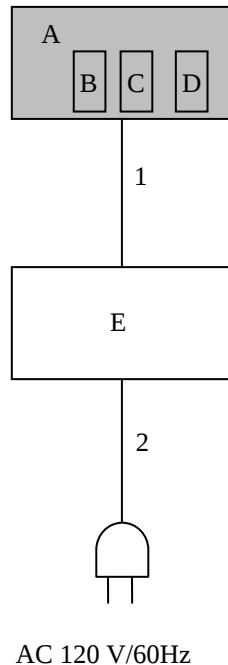
[Conducted emission]
