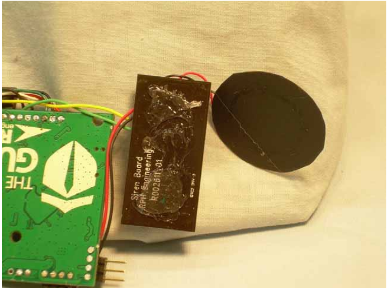
View of the Trace Side of the Siren PCB
