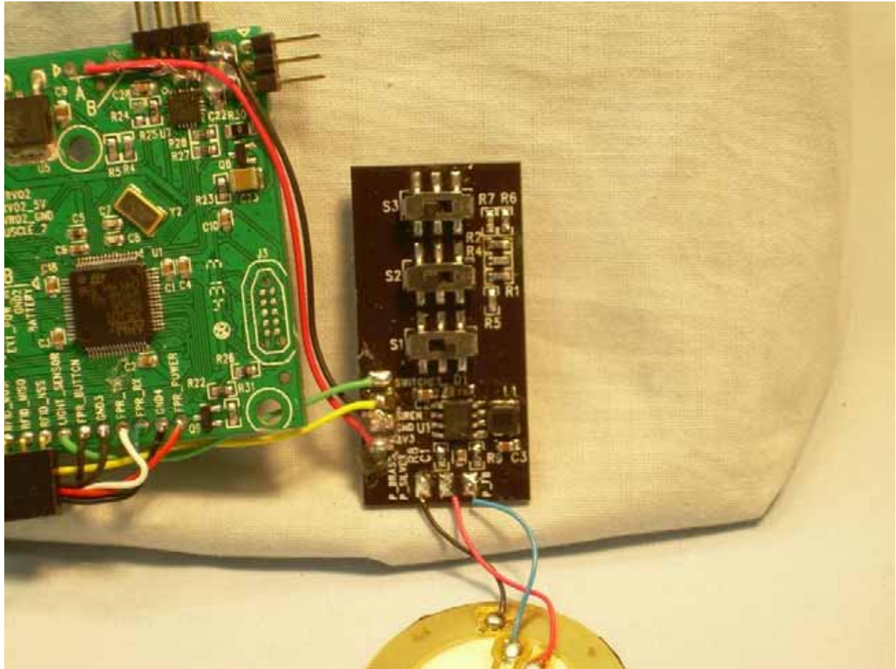
View of the Component Side of the Siren PCB
