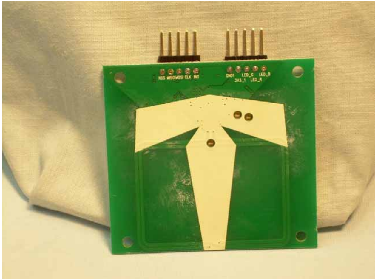
View of the Trace Side of the RFID PCB
