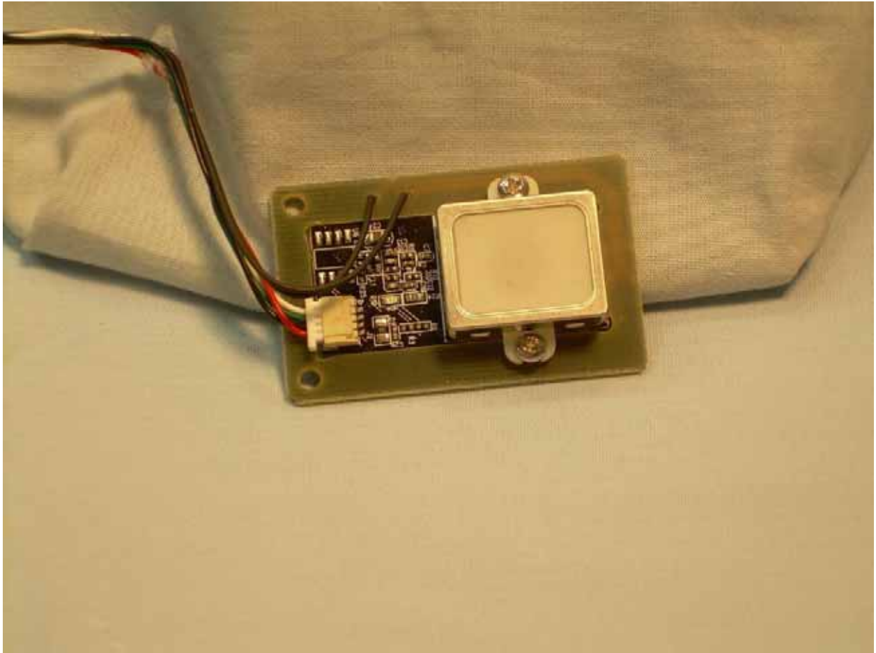
View of the Component Side of the Fingerprint PCB
