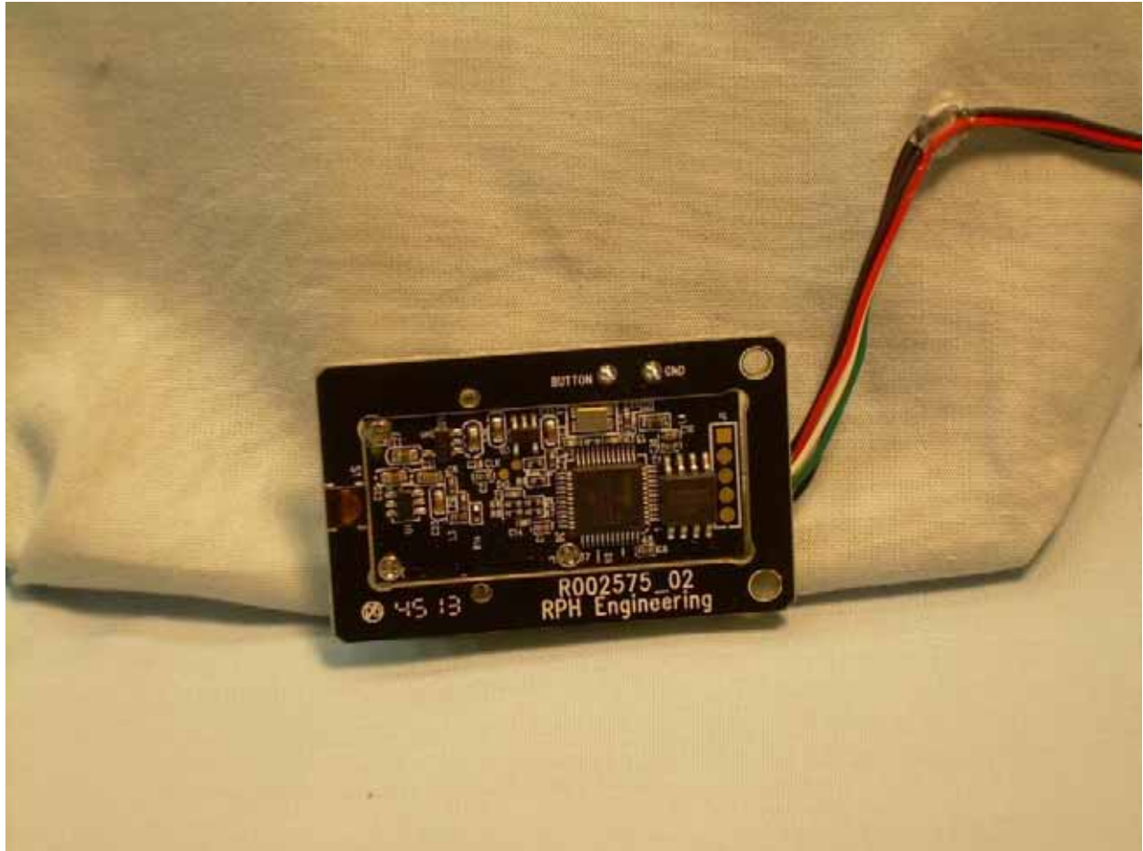
View of the Trace Side of the Fingerprint PCB
