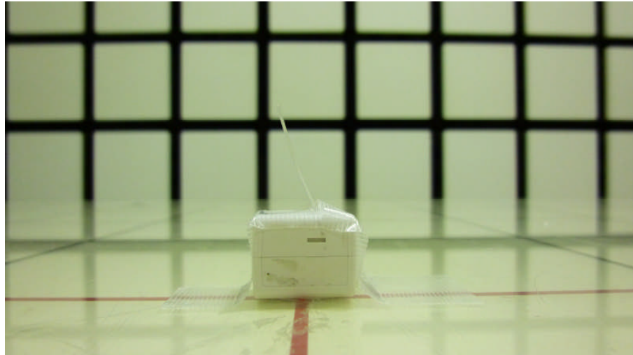
Photo1 EUT setup
