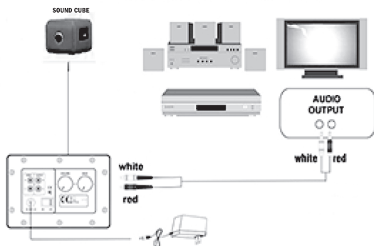
DIAGRAM 2 HOME THEATER & SATELLITE
