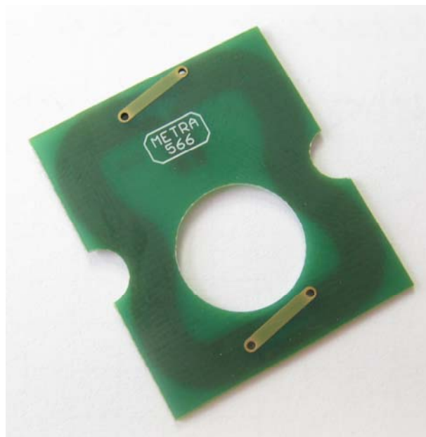
Figure 5: Door RFID Antenna – bottom side
