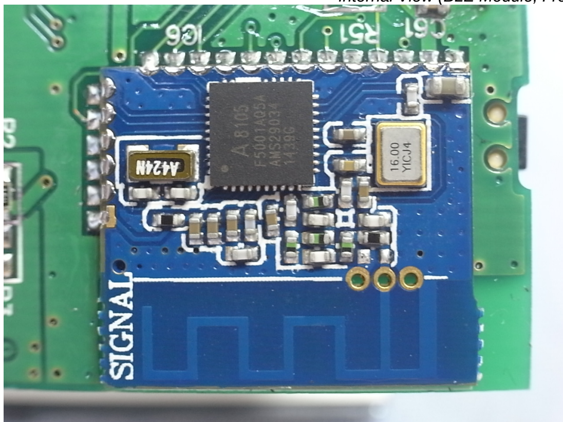
Figure 8 Internal View (BLE Module, Front View)
