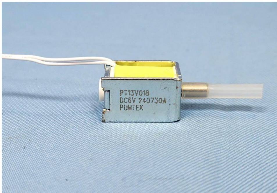
EUT Photo (22)
