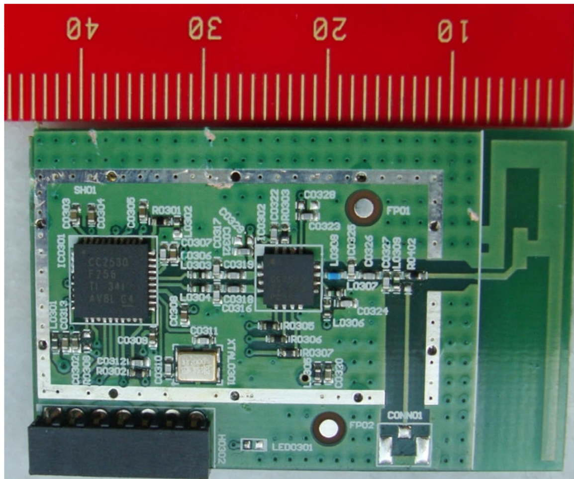
Front View, RF shielding removed
