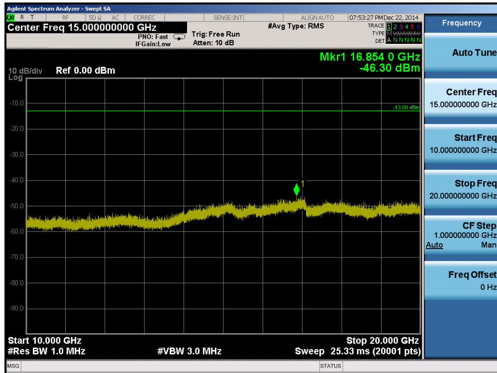
Plot 7-12. Conducted Spurious Plot (PCS CDMA Mode – Ch. 600)
