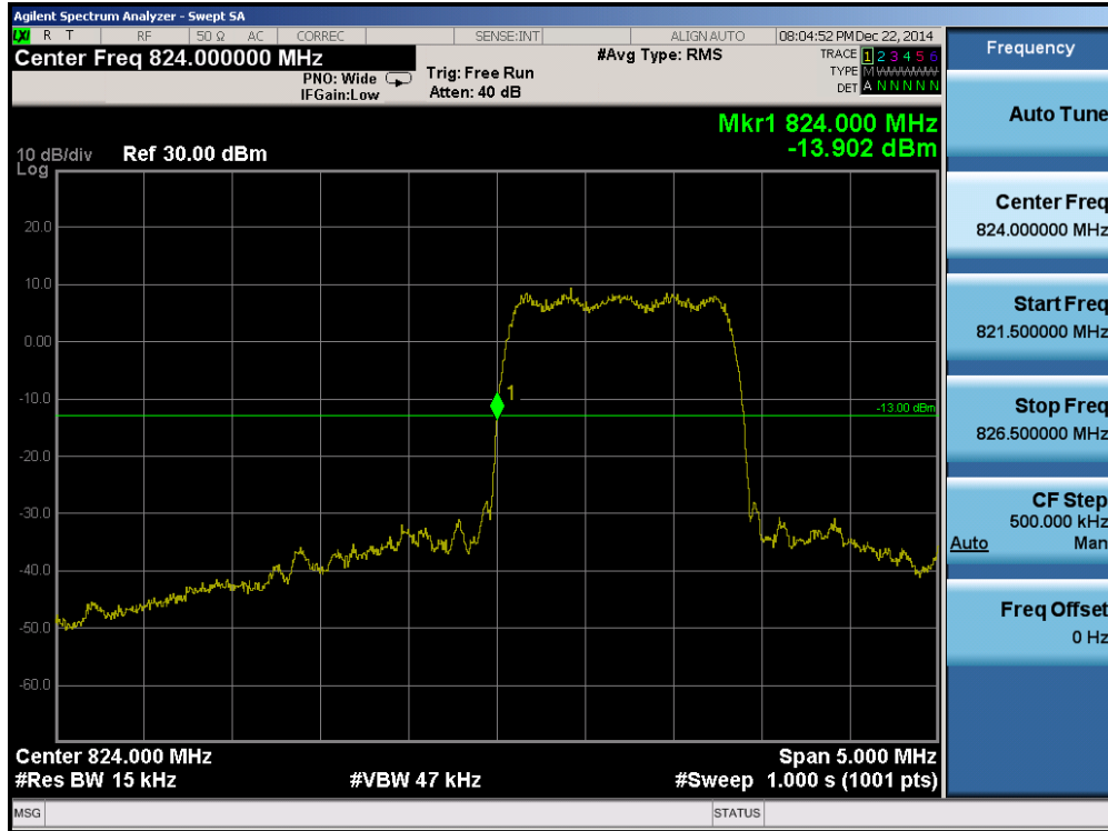
Plot 7-15. Band Edge Plot (Cellular CDMA Mode – Ch. 1013)
