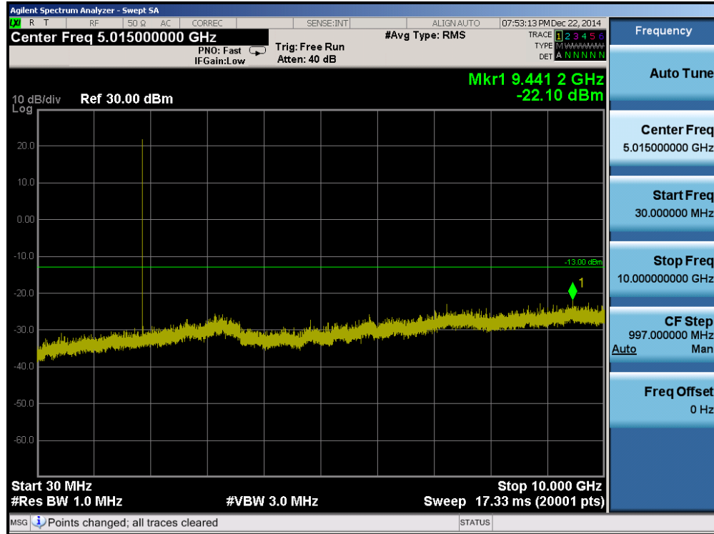
Plot 7-11. Conducted Spurious Plot (PCS CDMA Mode – Ch. 600)
