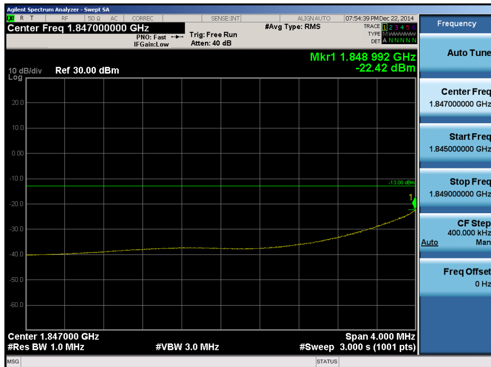
Plot 7-20. 4MHz Span Plot (PCS CDMA Mode – Ch. 25)
