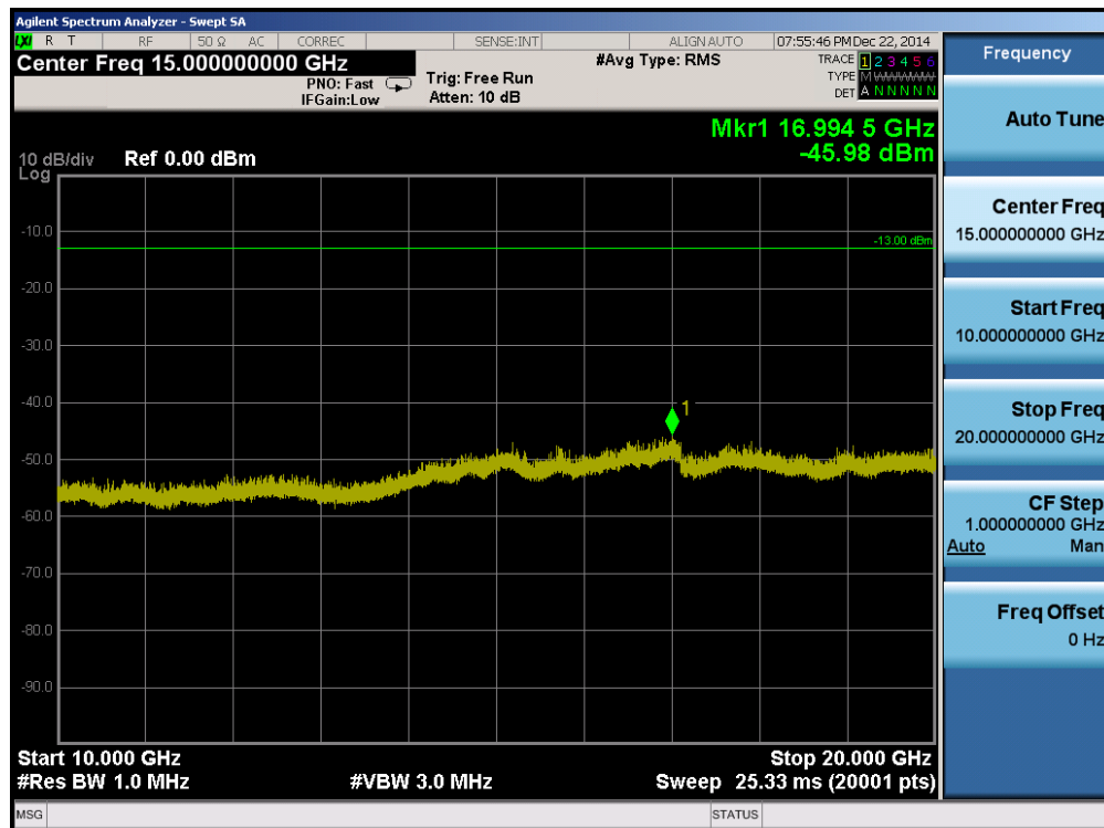
Plot 7-10. Conducted Spurious Plot (PCS CDMA Mode – Ch. 25)
