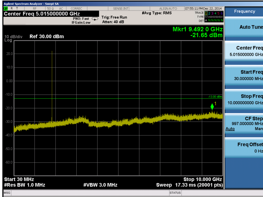
Plot 7-9. Conducted Spurious Plot (PCS CDMA Mode – Ch. 25)
