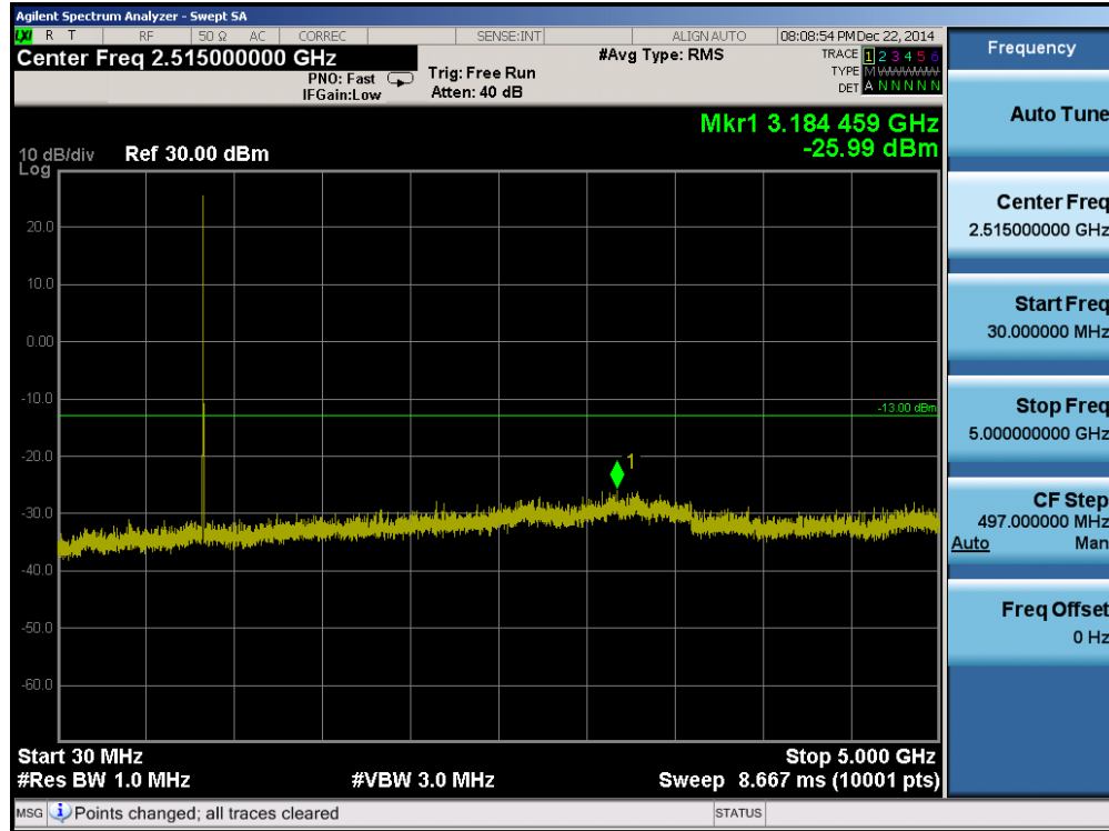
Plot 7-7. Conducted Spurious Plot (Cellular CDMA Mode – Ch. 777)
