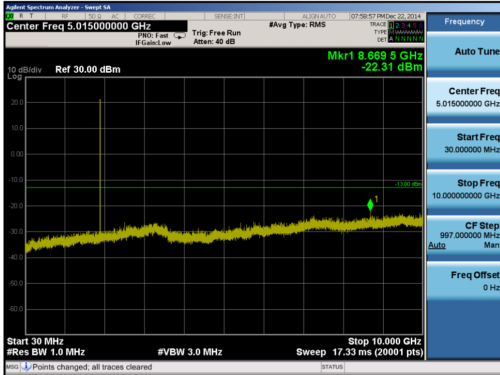
Plot 7-13. Conducted Spurious Plot (PCS CDMA Mode – Ch. 1175)
