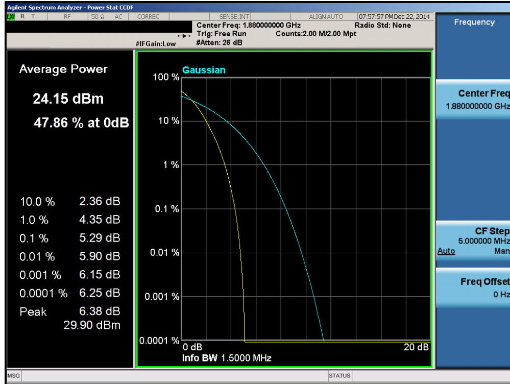
Plot 7-23. Peak-Average Ratio Plot (PCS CDMA Mode – Ch. 600)
