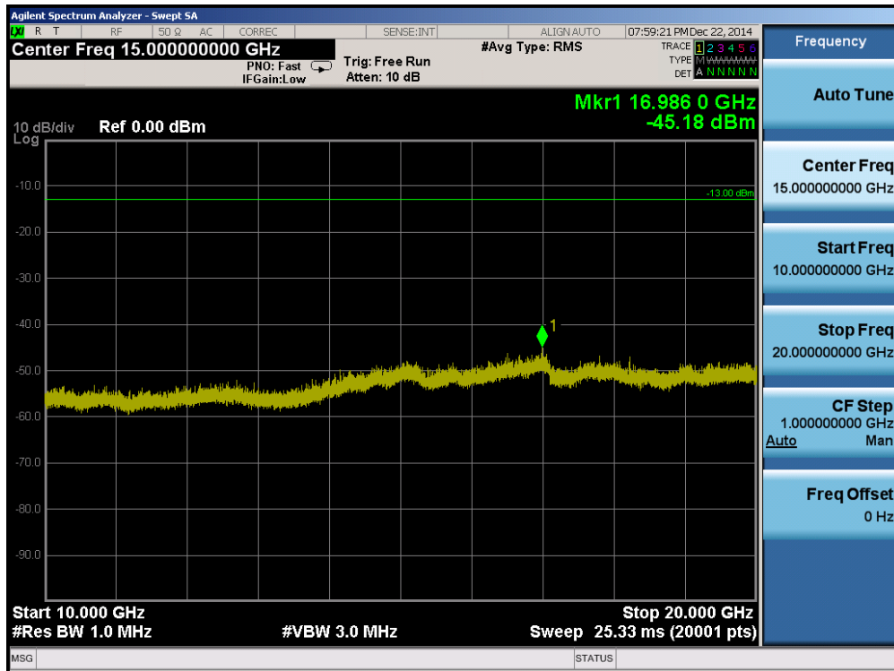
Plot 7-14. Conducted Spurious Plot (PCS CDMA Mode – Ch. 1175)
