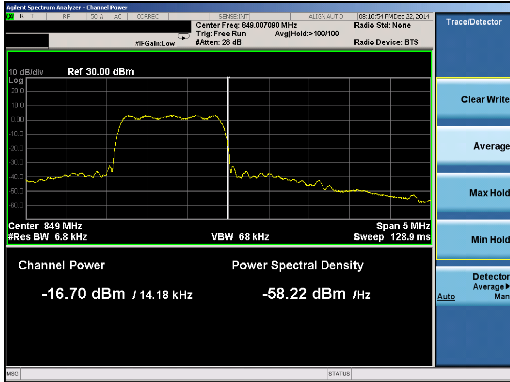
Plot 7-17. Band Edge Plot (Cellular CDMA Mode – Ch. 777)
