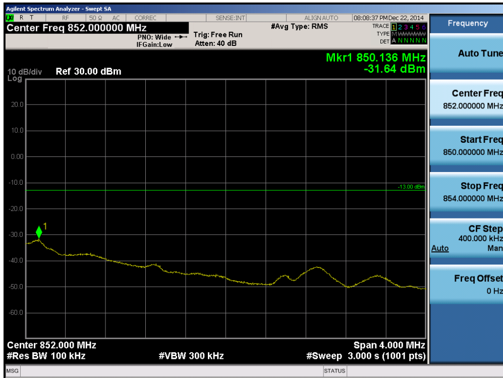
Plot 7-18. 4MHz Span Plot (Cellular CDMA Mode – Ch. 777)
