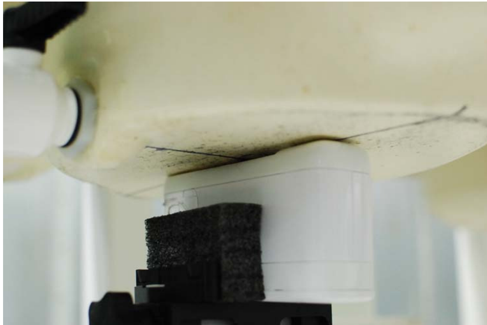
SAR Test Setup Photo 2: Front Side at 0.0 cm
