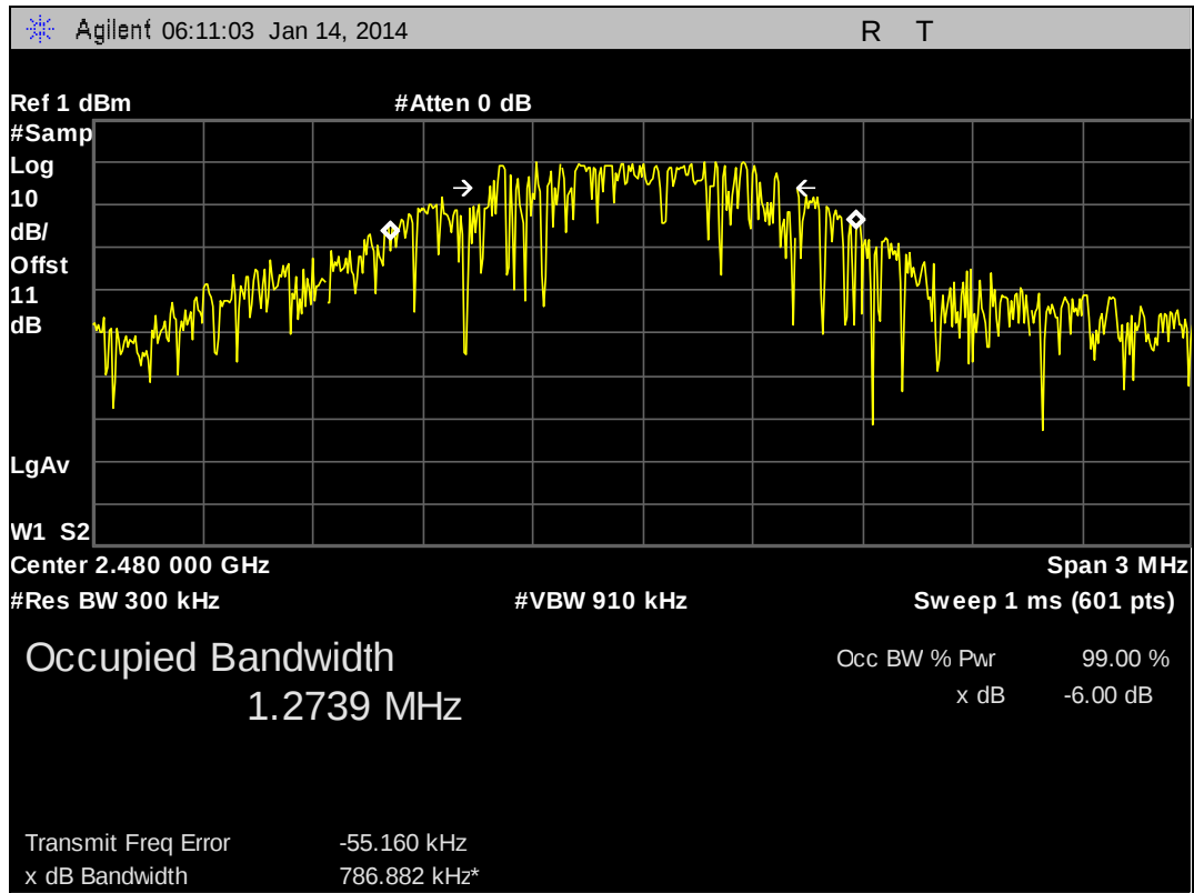
Plot 7. 99% Occupied Bandwidth, High Channel
