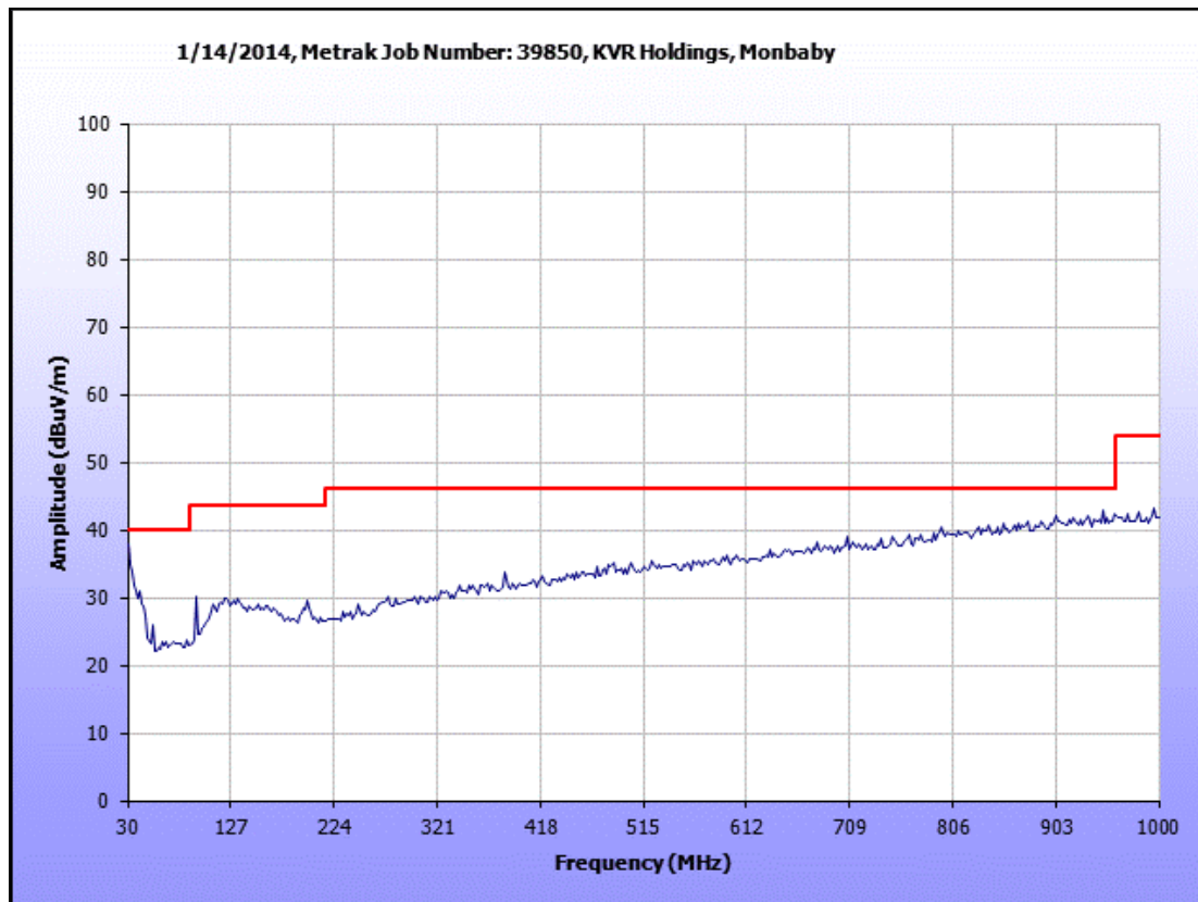
Plot 1. Radiated Emissions, 30 MHz - 1 GHz, FCC 15B & ICES-003 Limits
