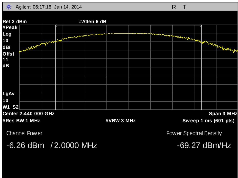
Plot 9. Peak Power Output, Mid Channel
