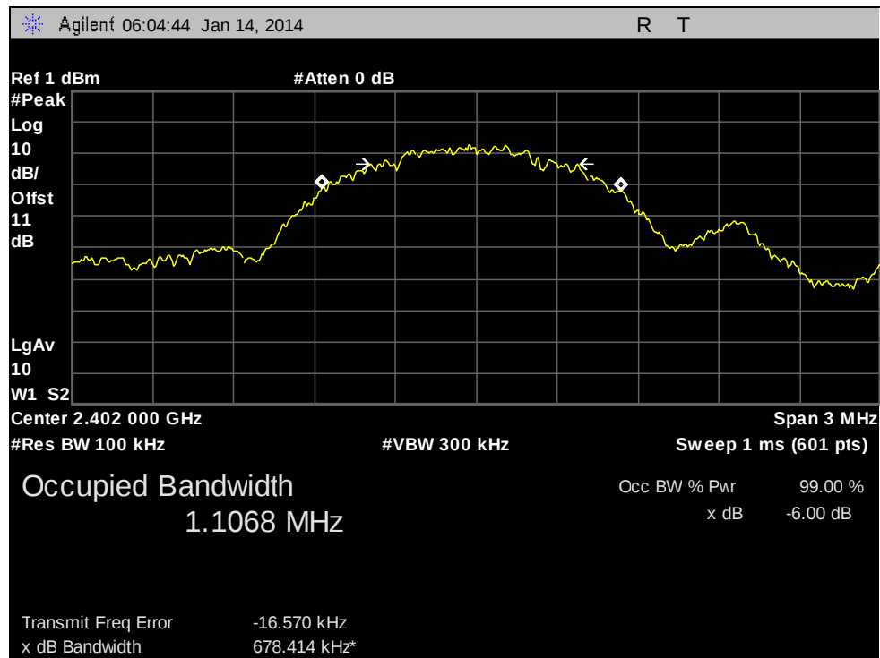
Plot 2. 6 dB Occupied Bandwidth, Low Channel
