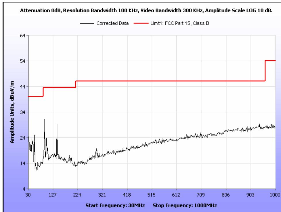
Plot 16. Radiated Spurious Emissions, Mid Channel, 30 MHz – 1 GHz, Peak
