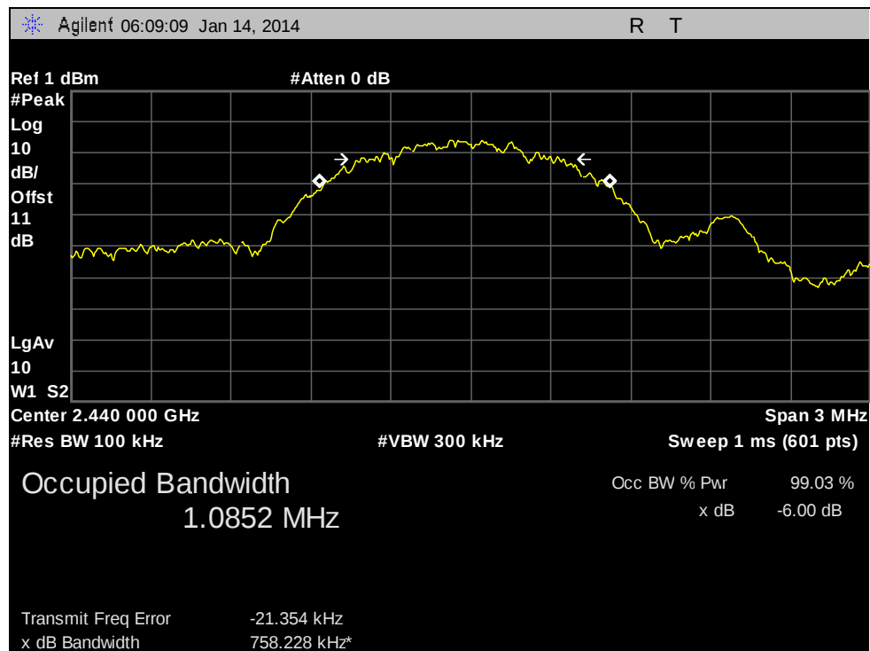
Plot 3. 6 dB Occupied Bandwidth, Mid Channel
