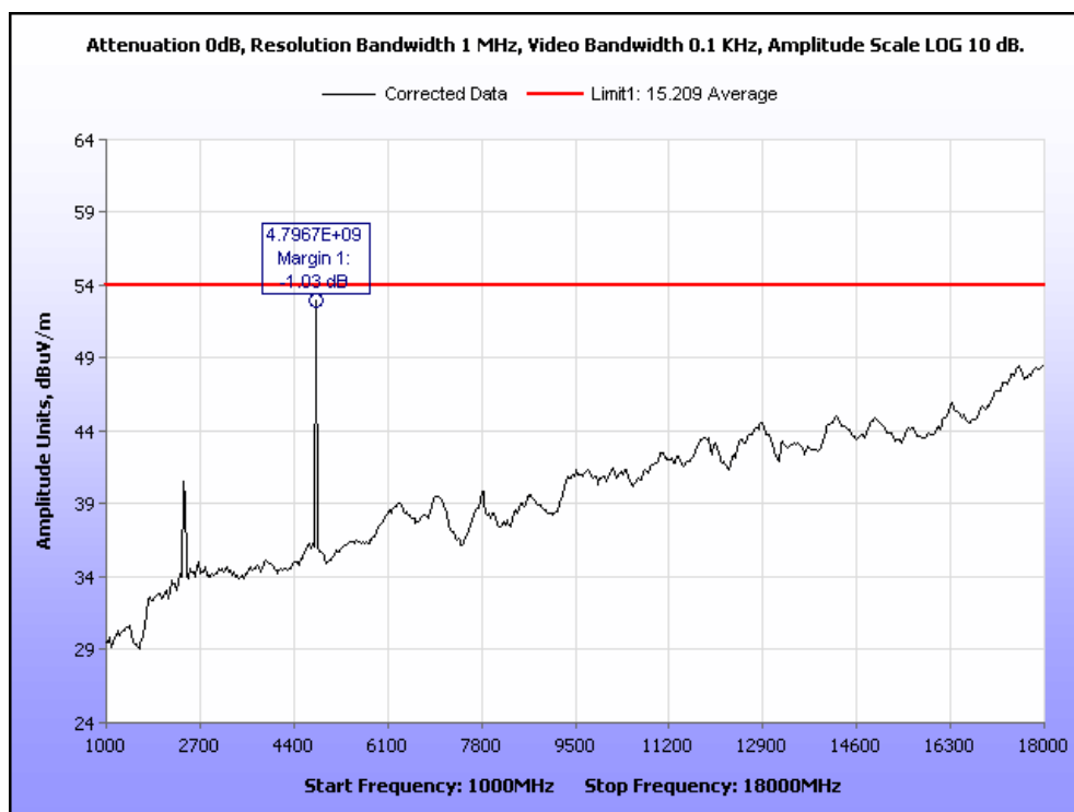
Plot 11. Radiated Spurious Emissions, Low Channel, 1 GHz – 18 GHz, Average
