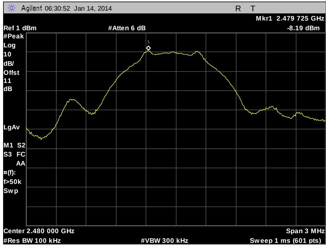
Plot 30. Peak Power Spectral Density, High Channel
