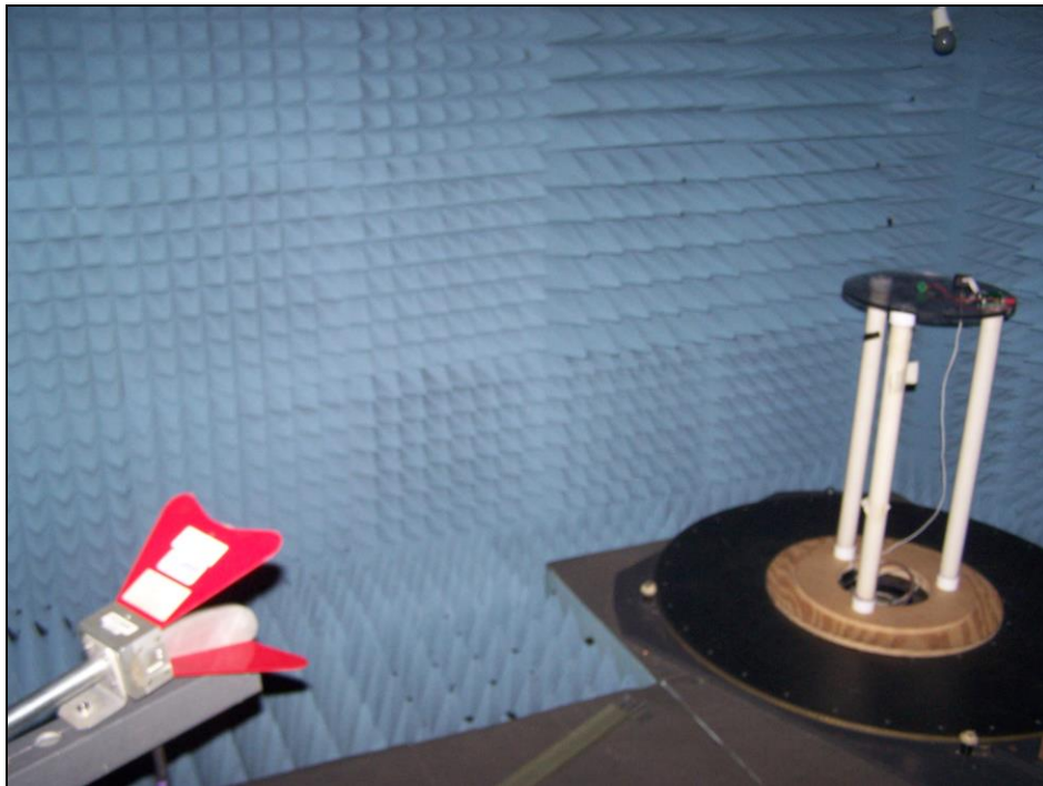
Photograph 4. Radiated Spurious Emissions, 1GHz-18GHz, Test Setup
