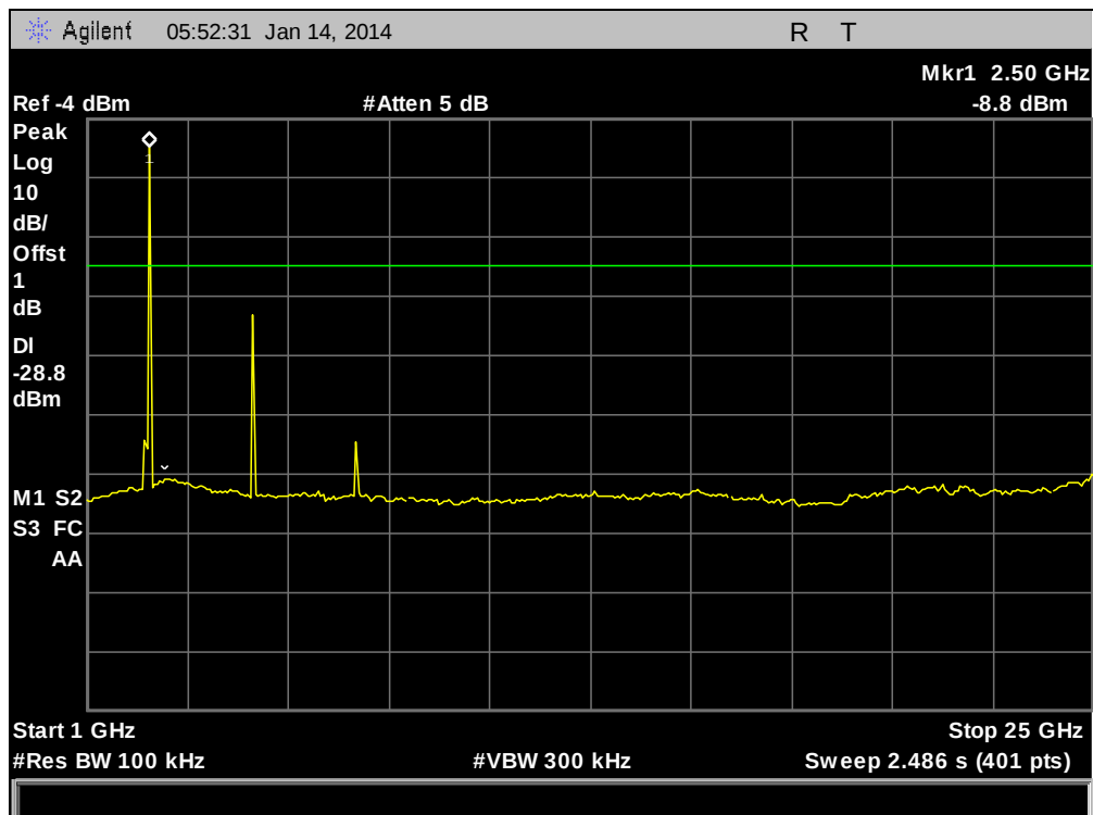
Plot 27. Conducted Spurious Emissions, High Channel, 1 GHz – 25 GHz
