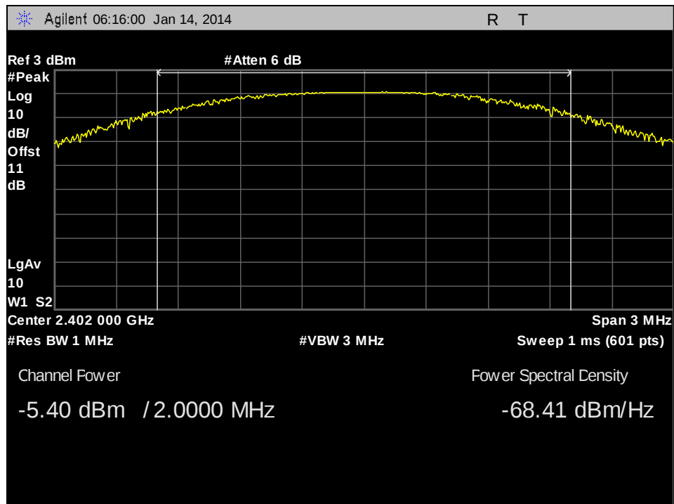
Plot 8. Peak Power Output, Low Channel
