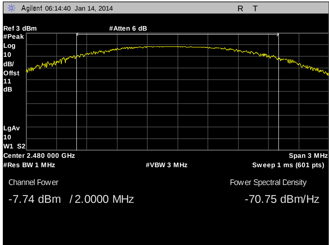
Plot 10. Peak Power Output, High Channel
