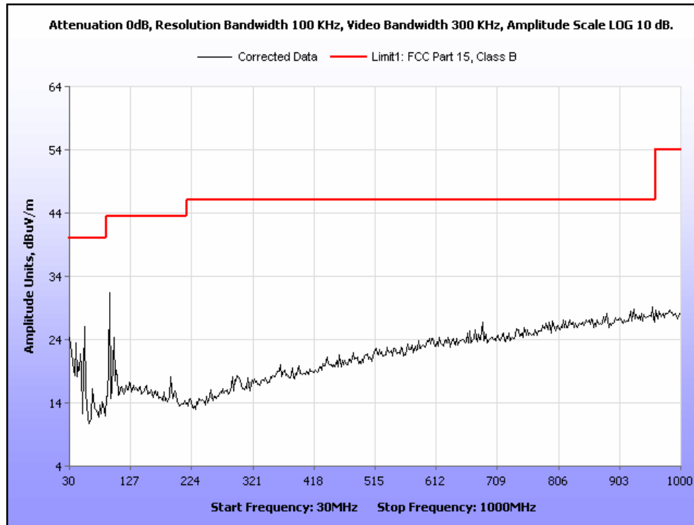
Plot 13. Radiated Spurious Emissions, Low Channel, 30 MHz – 1 GHz, Peak
