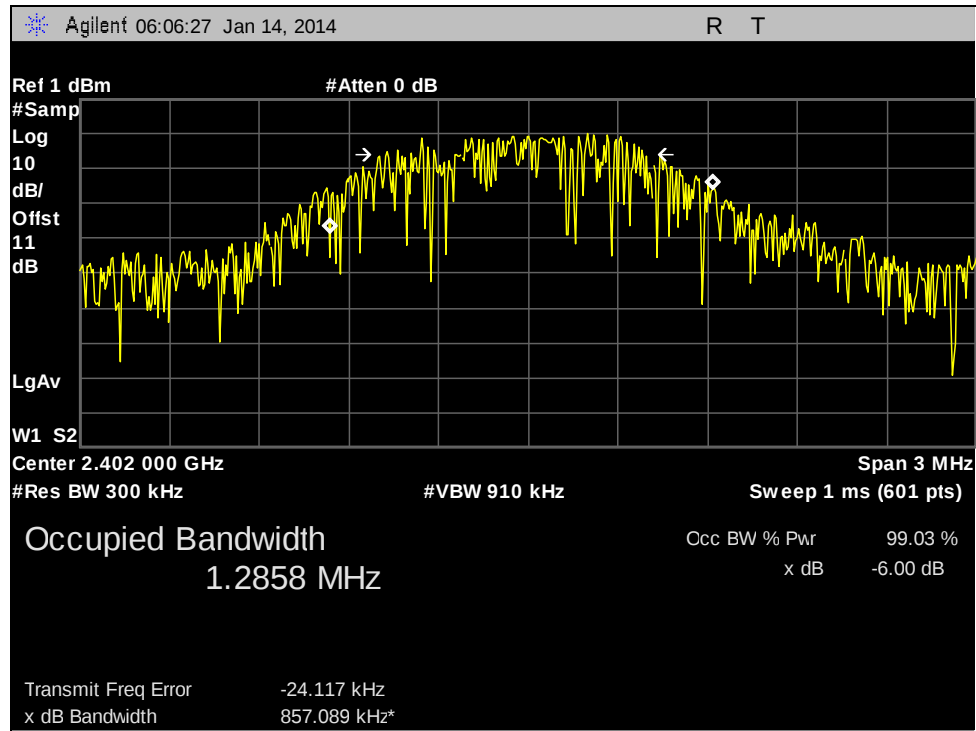
Plot 5. 99% Occupied Bandwidth, Low Channel
