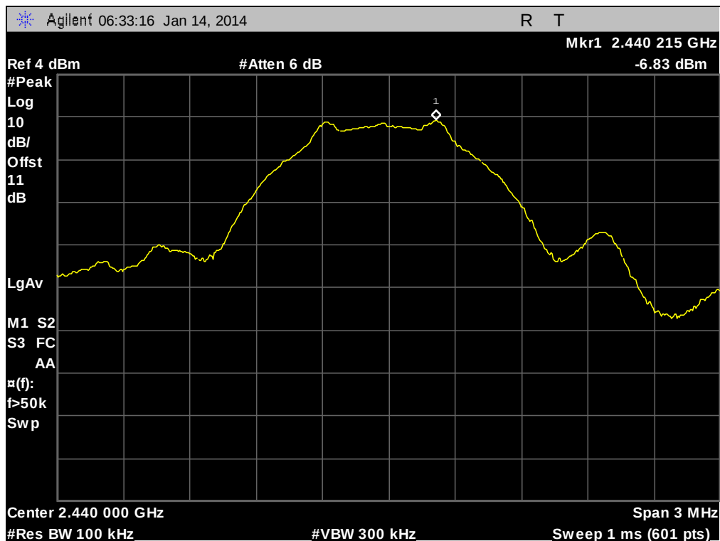
Plot 29. Peak Power Spectral Density, Mid Channel
