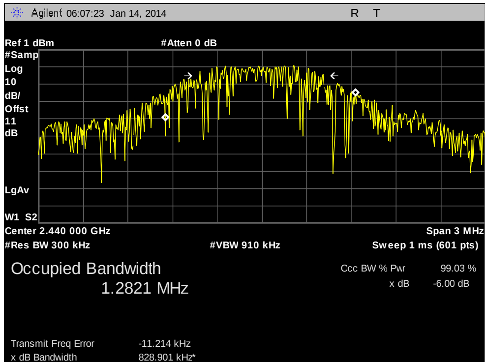
Plot 6. 99% Occupied Bandwidth, Mid Channel
