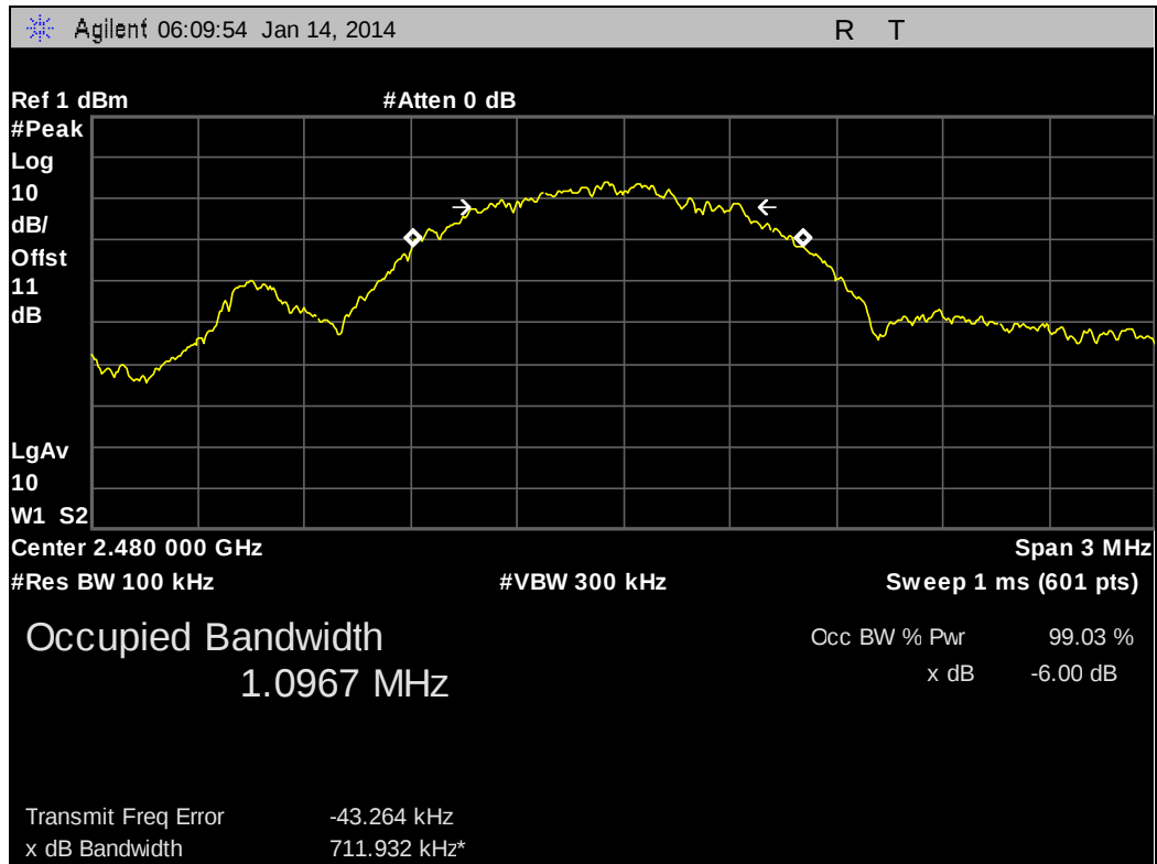
Plot 4. 6 dB Occupied Bandwidth, High Channel
