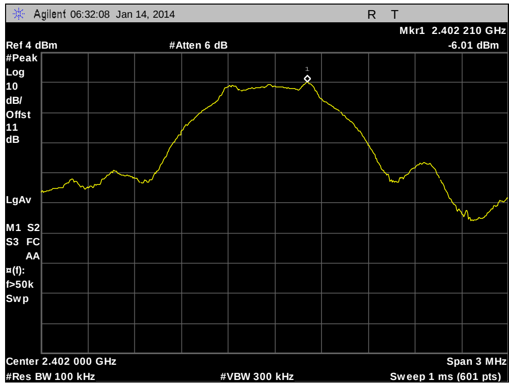
Plot 28. Peak Power Spectral Density, Low Channel
