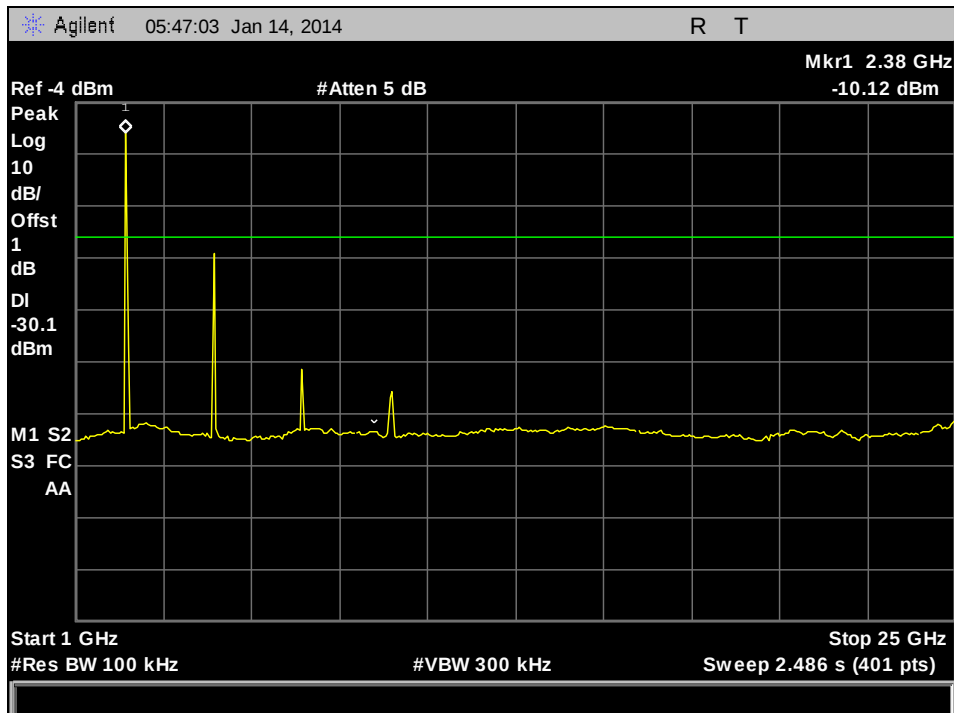
Plot 23. Conducted Spurious Emissions, Low Channel, 1 GHz – 25 GHz
