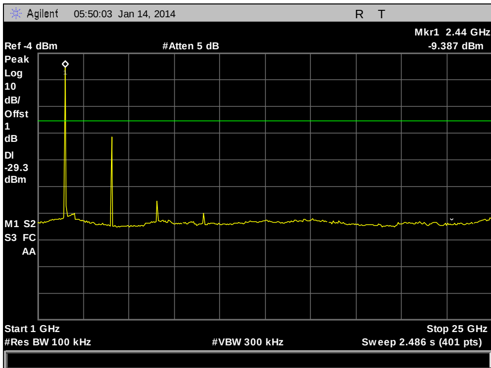
Plot 25. Conducted Spurious Emissions, Mid Channel, 1 GHz – 25 GHz
