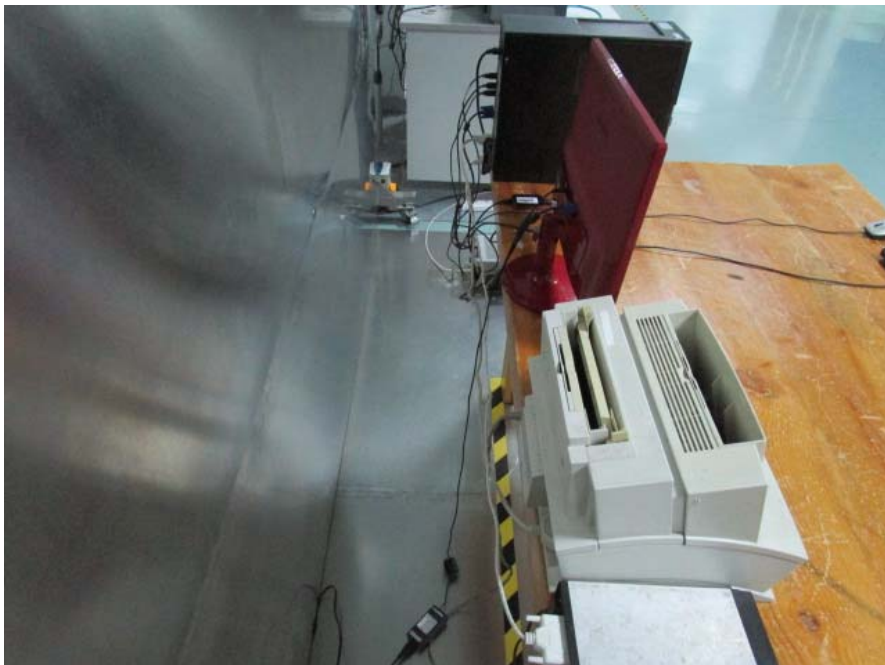
Conducted Emission - Side View (Terminal Antenna)
