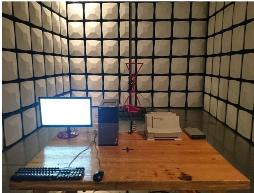
Radiated Emission - Front View (Below 1GHz) (Terminal Antenna)
