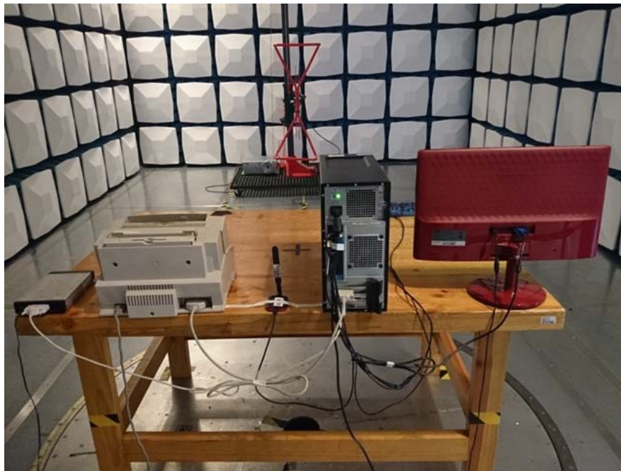
Radiated Emission - Rear View (Below 1GHz) (Terminal Antenna)
