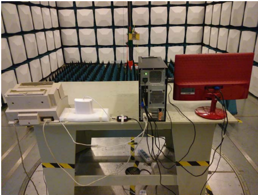
Radiated Emission - Rear View (Above 1GHz) (Wall Mount Antenna)
