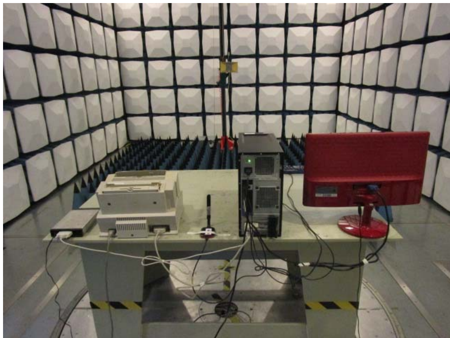
Radiated Emission - Rear View (Above 1GHz) (Terminal Antenna)
