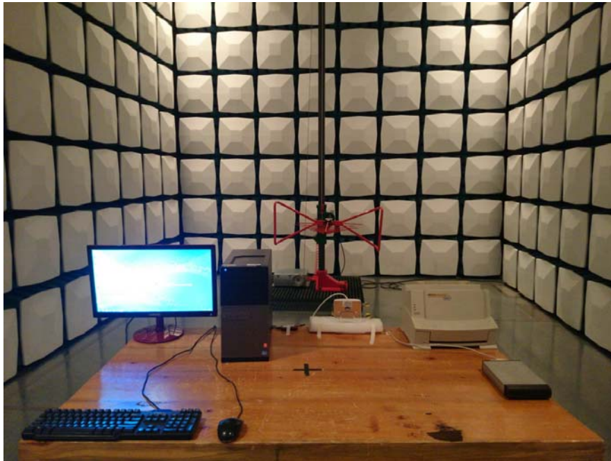
Radiated Emission - Front View (Below 1GHz) (Wall Mount Antenna)
