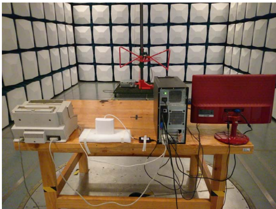
Radiated Emission - Rear View (Below 1GHz) (Wall Mount Antenna)
