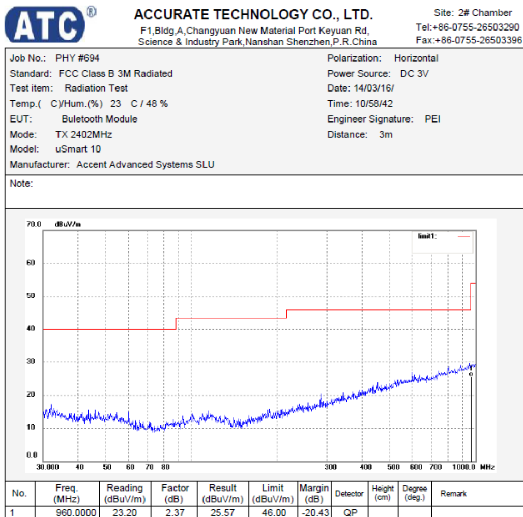
Figure 3: Test figure of spurious emissions, mode A.1, Horizontal polarity (30MHz – 1GHz)
