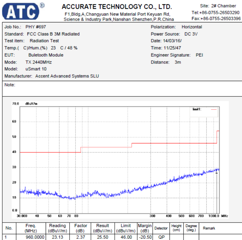
Figure 11: Test figure of spurious emissions, mode A.2, Horizontal polarity (30MHz – 1GHz)
