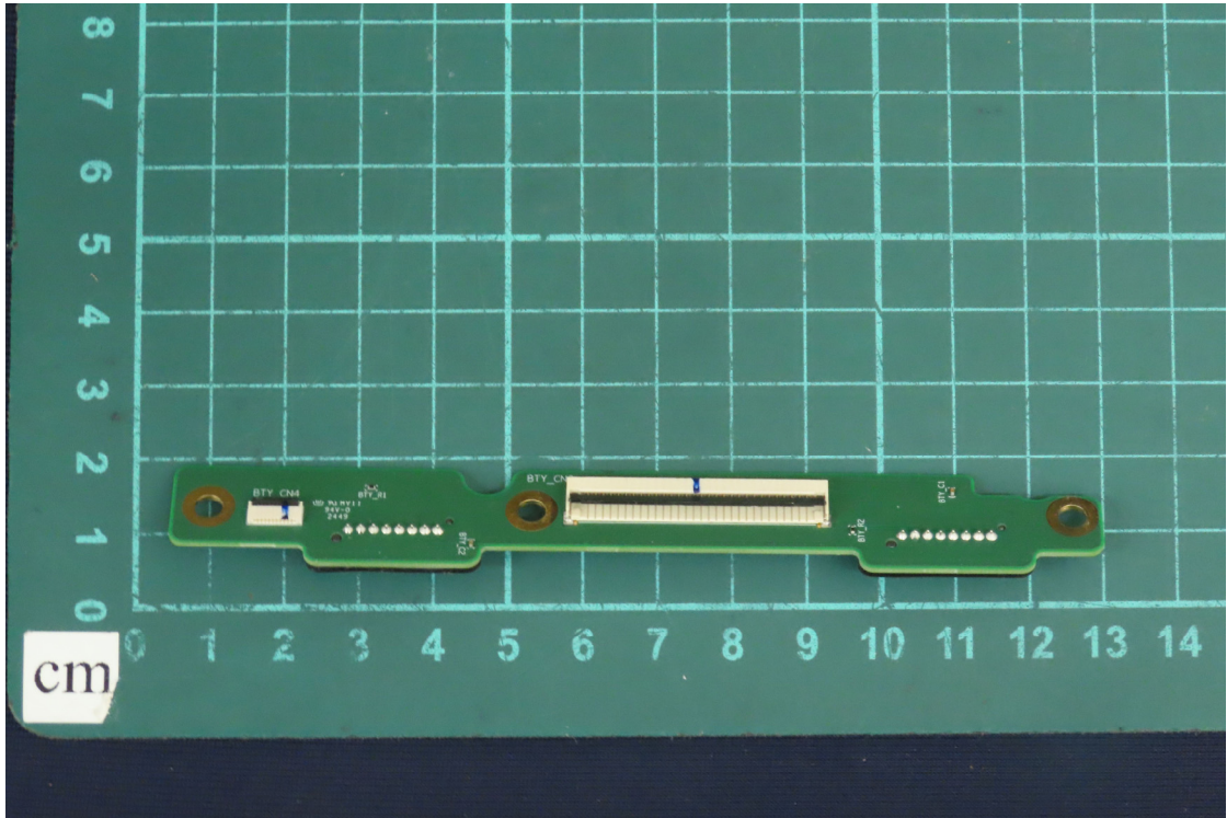
(27) EUT Photo
