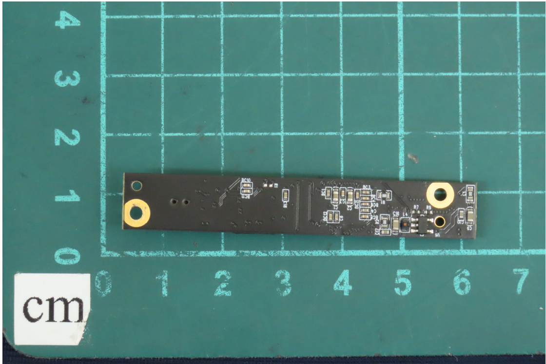
(29) EUT Photo
