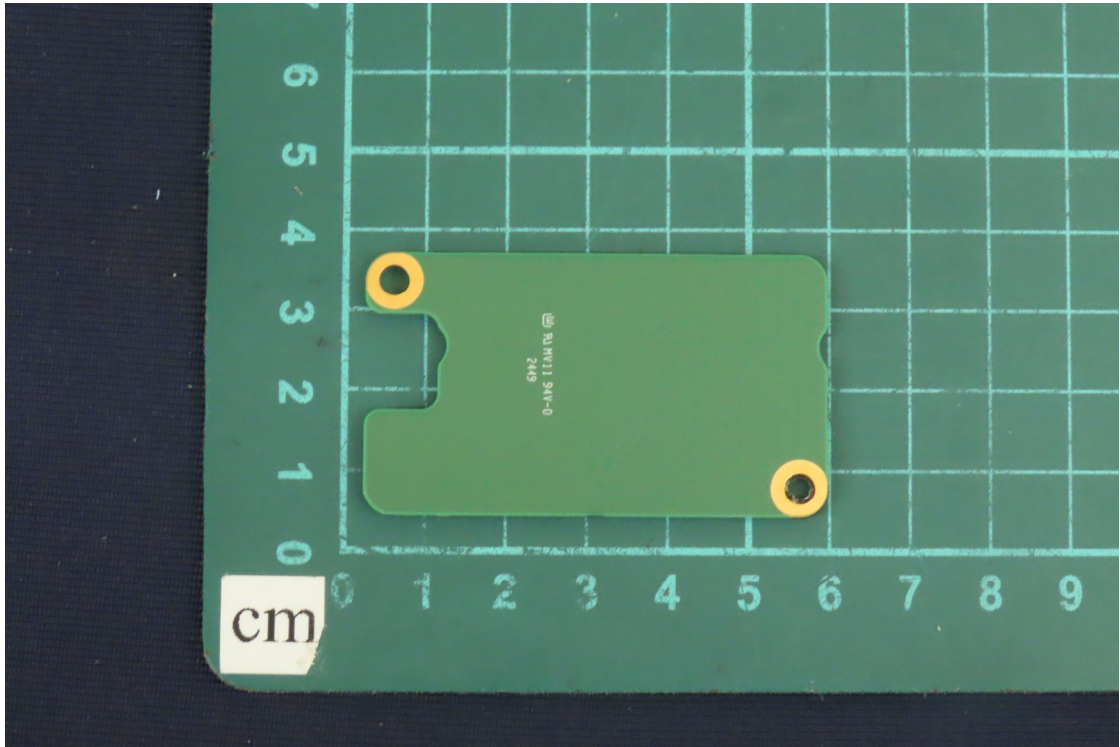
(25) EUT Photo
