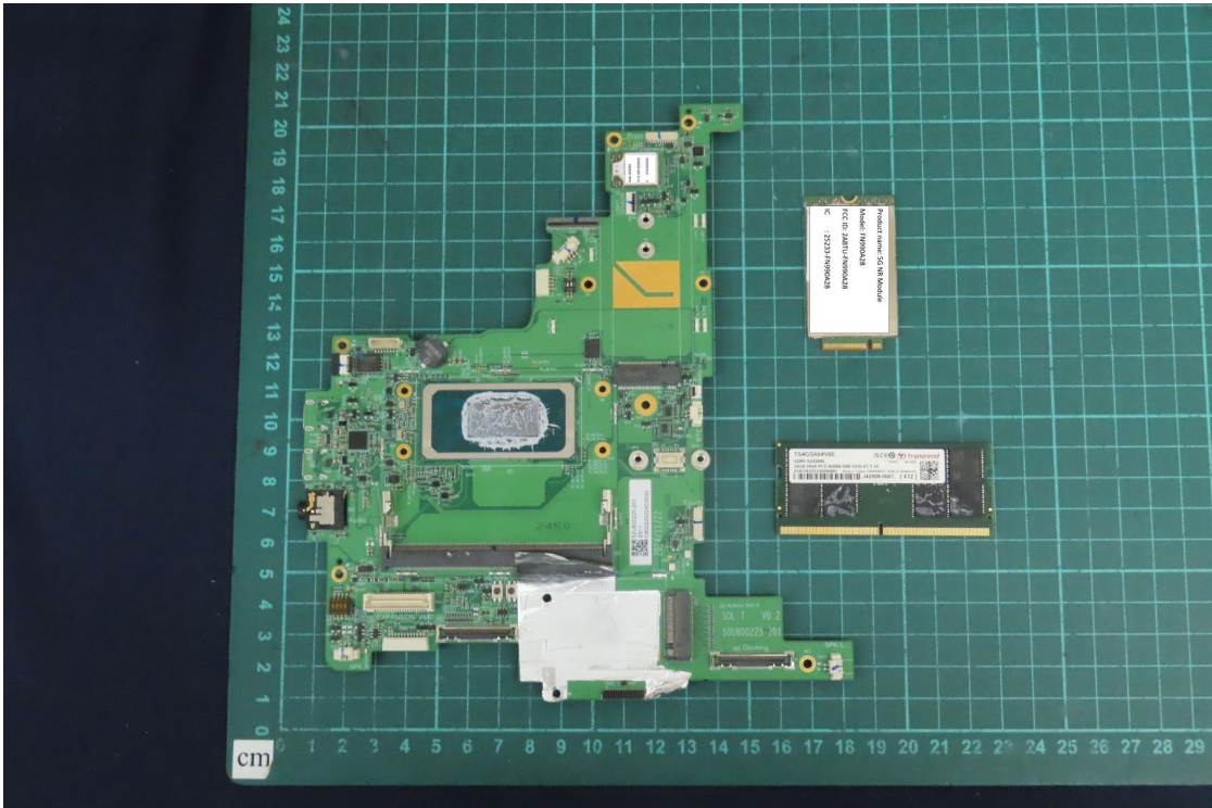
(34) EUT Photo
