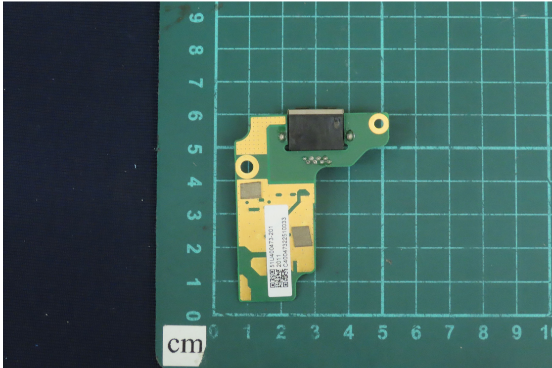
(32) EUT Photo
