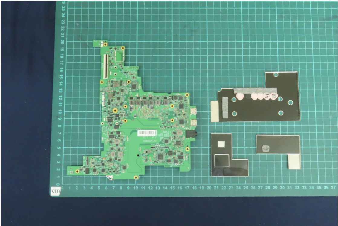
(43) EUT Photo
