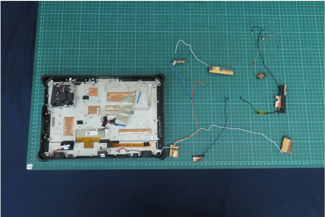
(51) EUT Photo
