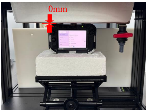
Photograph 3. Body, Top Edge, 0mm
