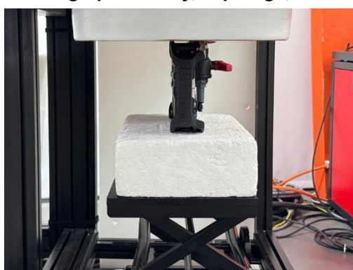
Photograph 6. Body, Bottom Edge, 0mm
