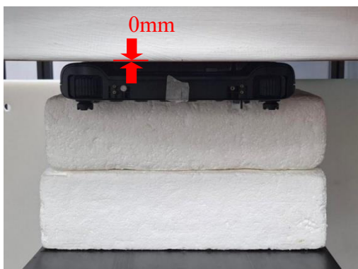
Photograph 1. Body, Back Surface, 0mm
