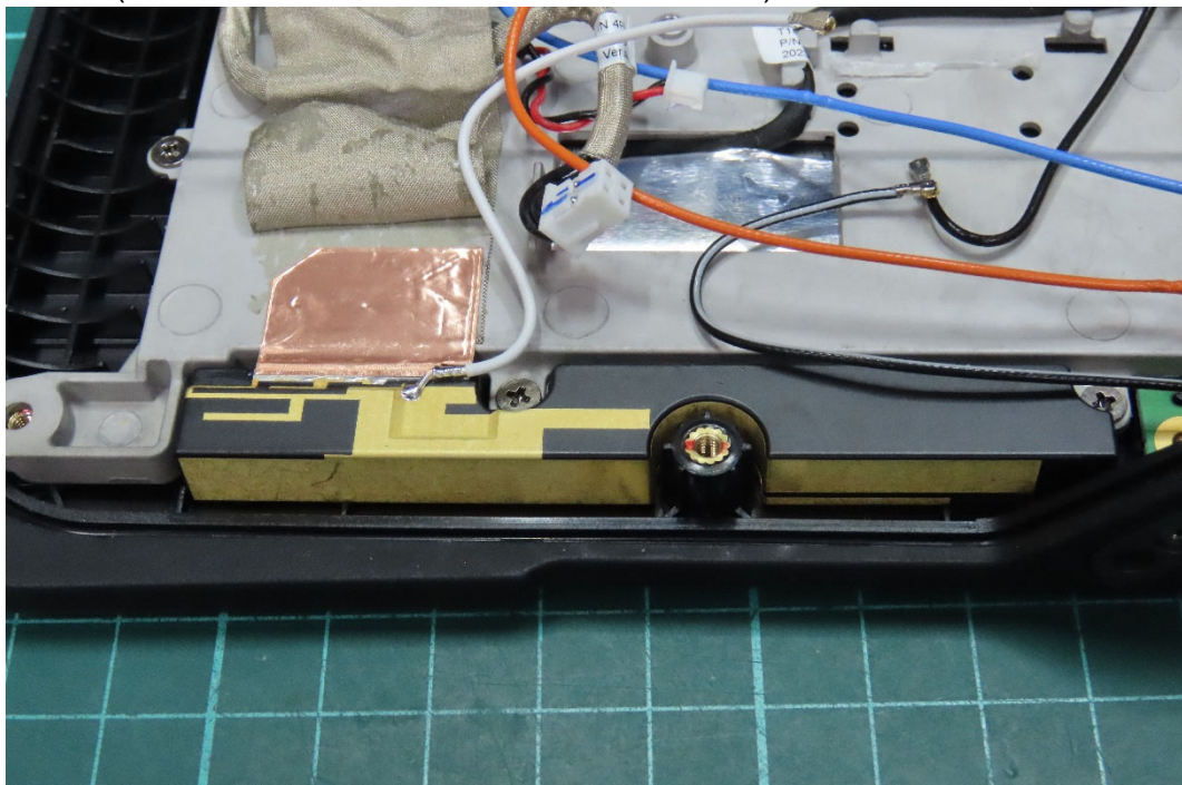
(34) EUT Photo (Model: ALL6Y-100005, WWAN Aux Antenna)
