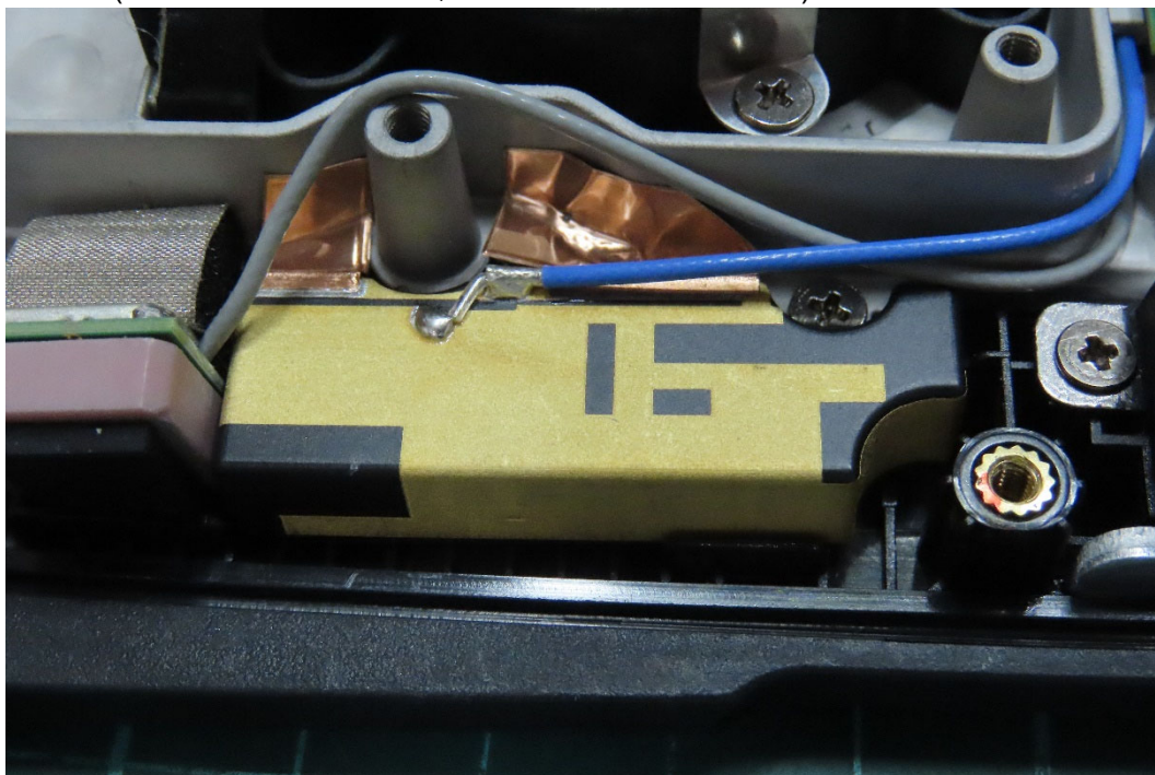
(31) EUT Photo (Model: ALL6Y-100004, WWAN MIMO1 Antenna)
