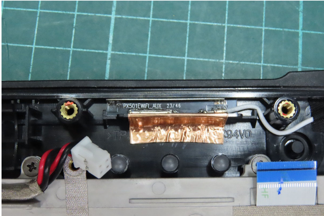
(29) EUT Photo (Model: ALP6Y-100003, WIFI Aux Antenna)
