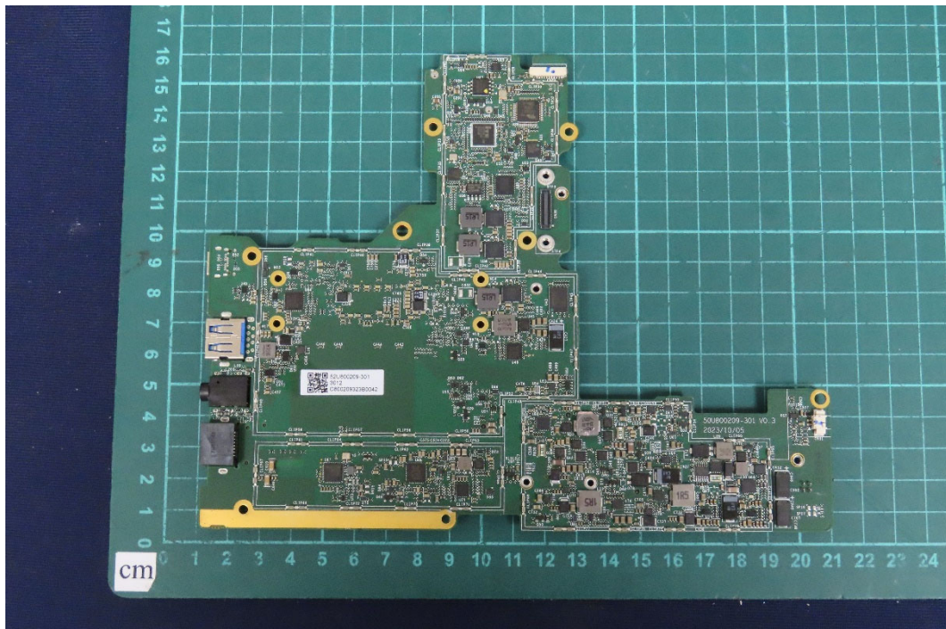
(26) EUT Photo
