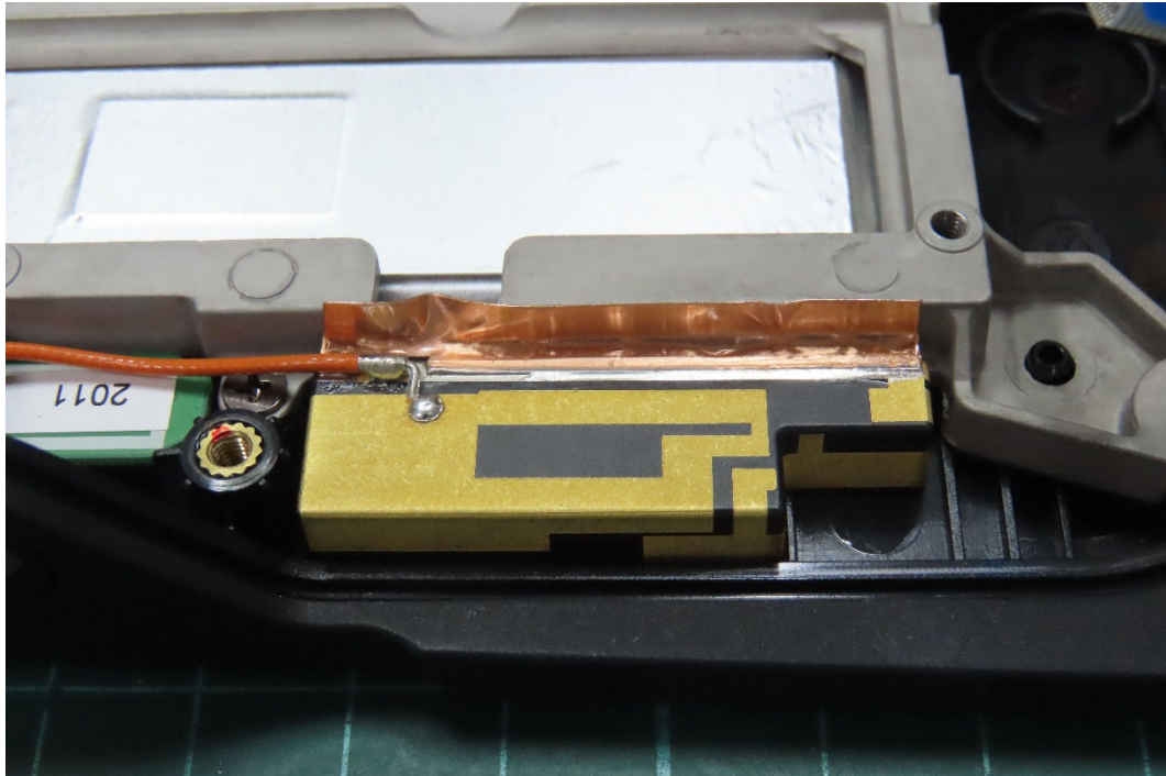
(33) EUT Photo (Model: ALL6Y-100006, WWAN MIMO2 Antenna)
