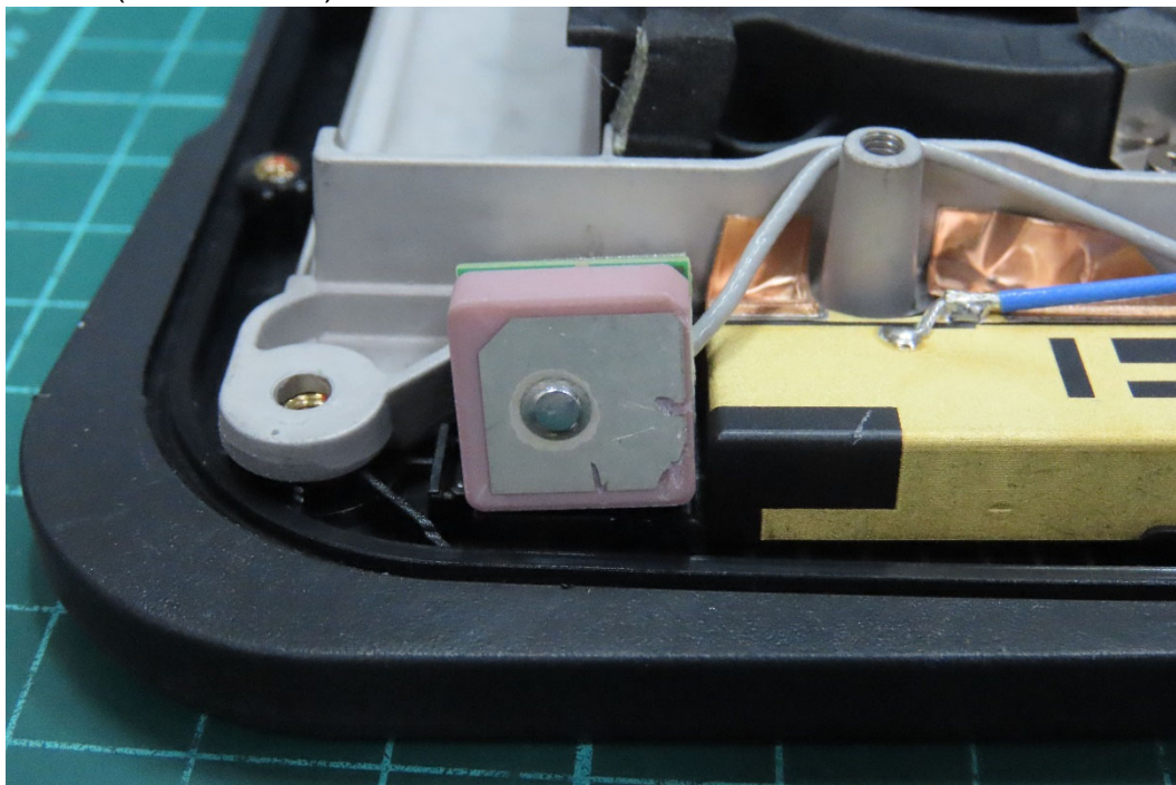
(32) EUT Photo (GPS Antenna)
