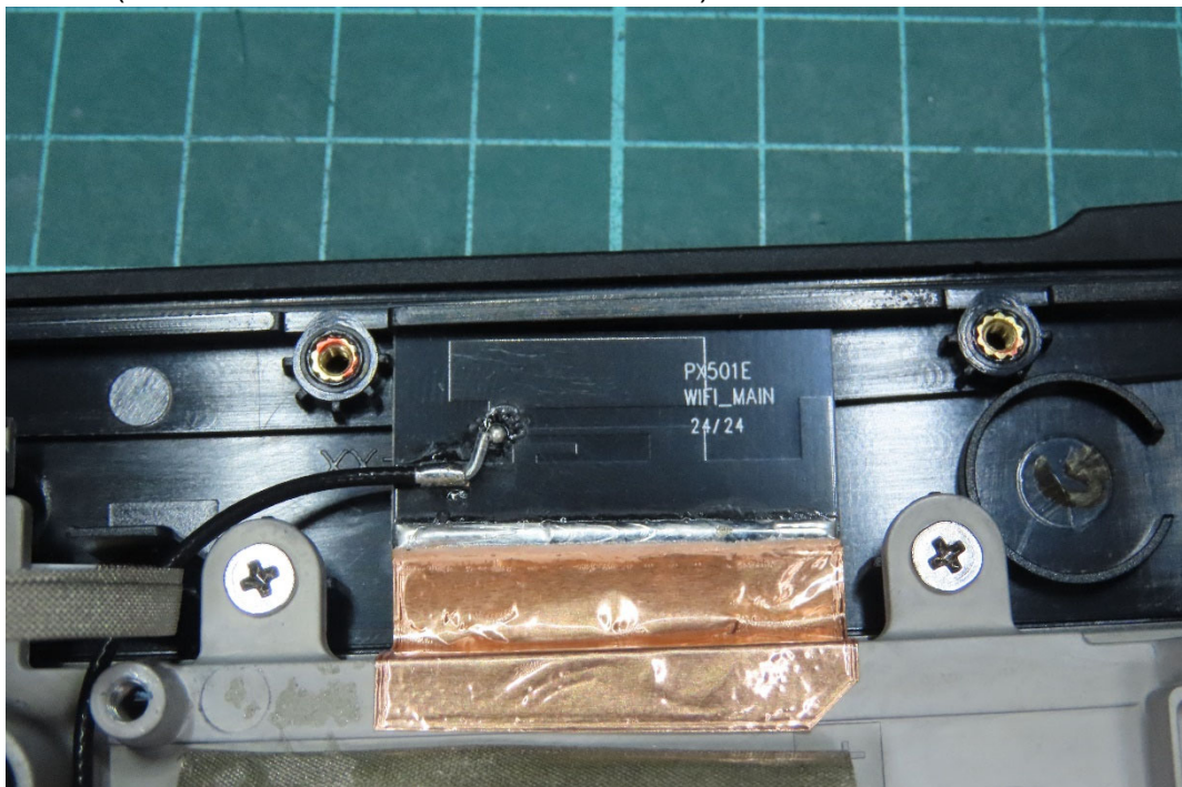
(28) EUT Photo (Model: ALP6Y-100002, WIFI Main Antenna)
