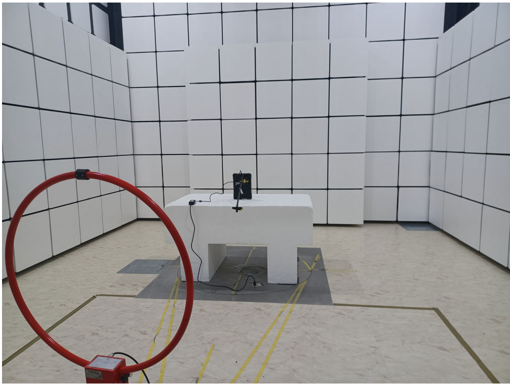
Radiated Test
