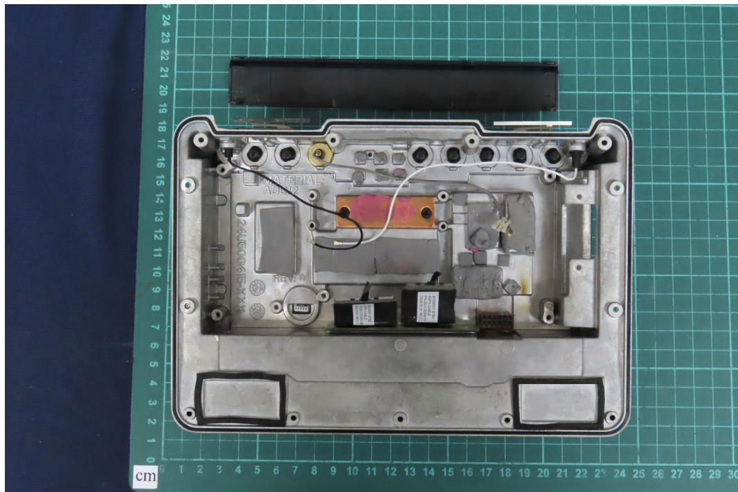
(45) EUT Photo
