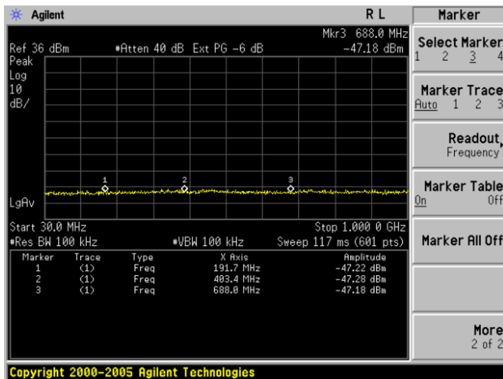
Conducted Emission Transmitting Mode CH 9400 30MHz – 1GHz
