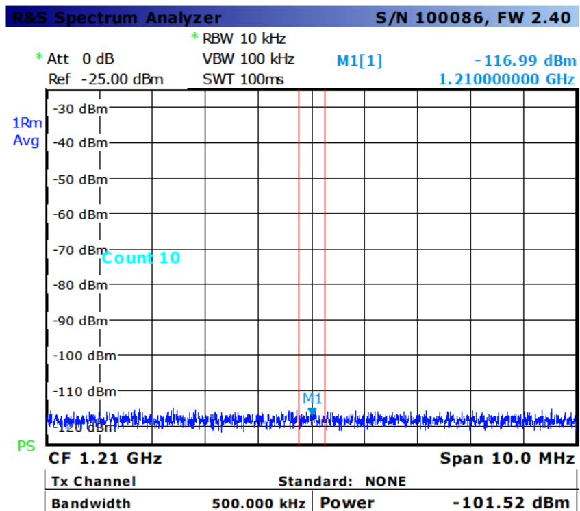
Figure 9--2 nd Harmonic Energy
