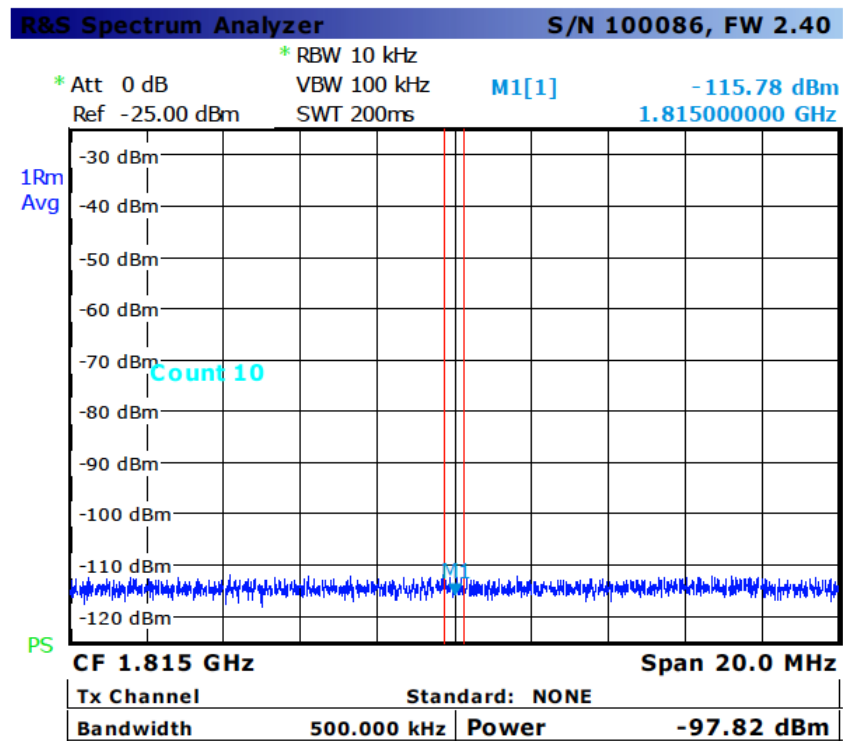
Figure 10—3 rd Harmonic Energy
